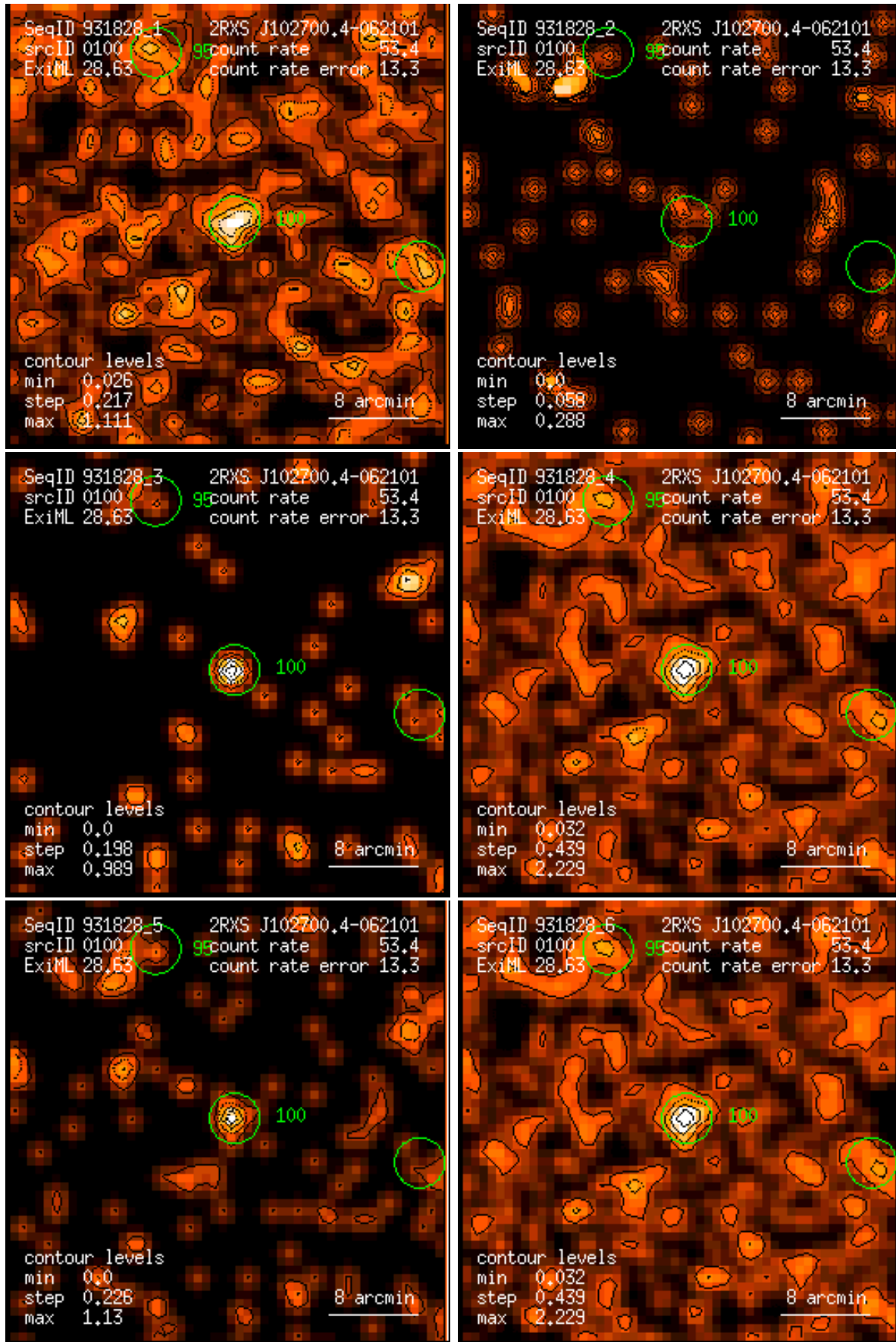
Figure 100: RASS 931828: detection 0100: band rate images, Gaussian filter: (1) PSPC channels 11 – 41, (2) 52 – 90, (3) 91 – 201, (4) 11 – 235, (5) 52 – 201, (6) 11 – 201. Broad band rates in counts/ks. Band rate contour levels in counts/ks/arcmin 2 .
