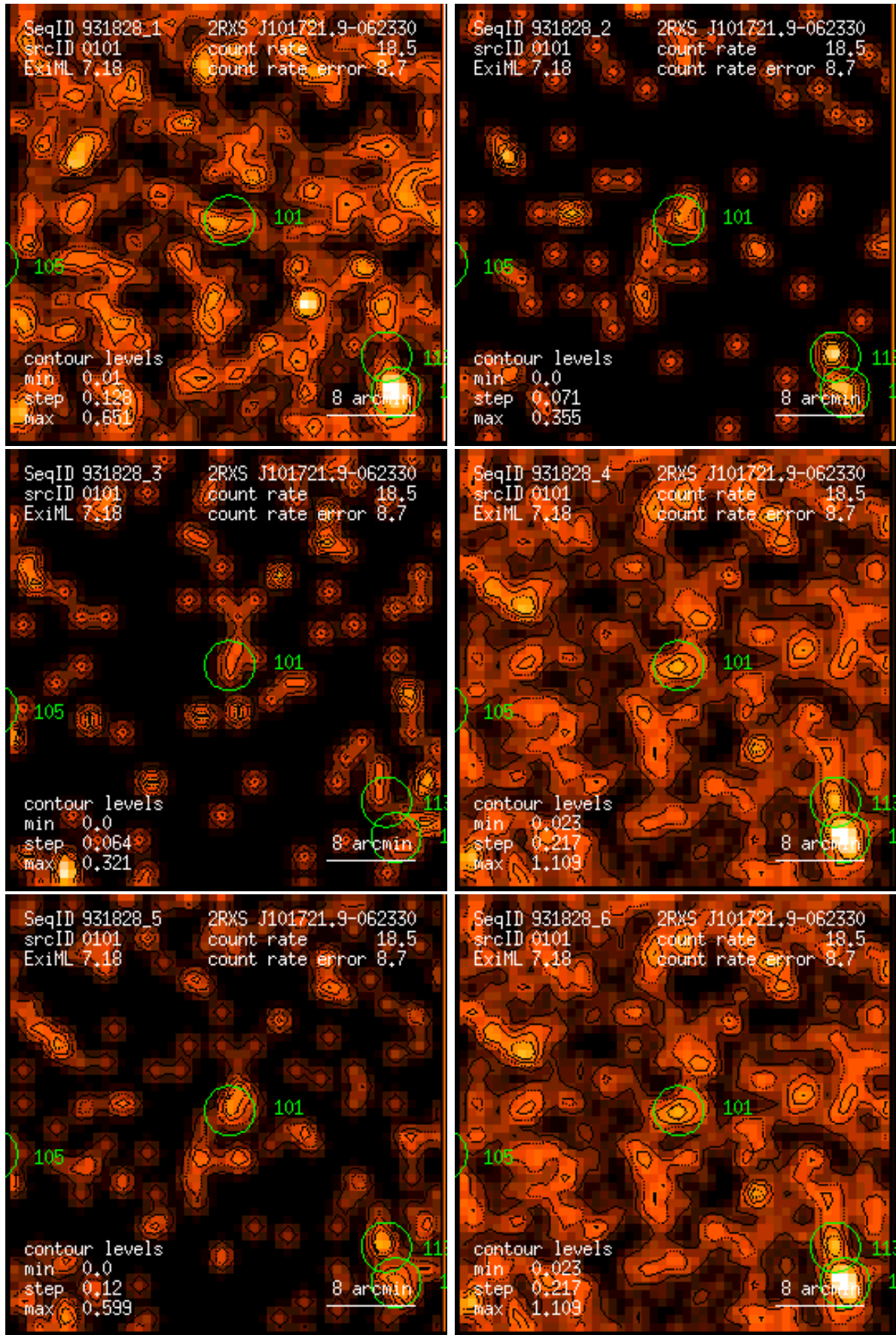
Figure 101: RASS 931828: detection 0101: band rate images, Gaussian filter: (1) PSPC channels 11 – 41, (2) 52 – 90, (3) 91 – 201, (4) 11 – 235, (5) 52 – 201, (6) 11 – 201. Broad band rates in counts/ks. Band rate contour levels in counts/ks/arcmin 2 .
