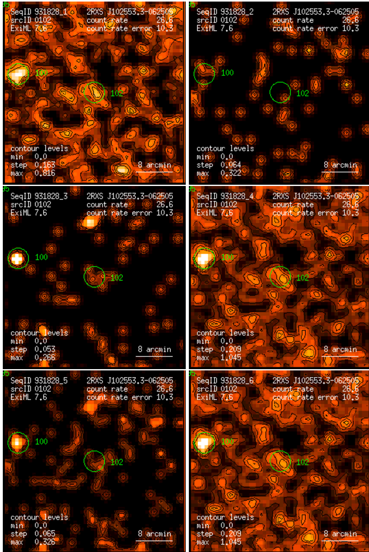
Figure 102: RASS 931828: detection 0102: band rate images, Gaussian filter: (1) PSPC channels 11 – 41, (2) 52 – 90, (3) 91 – 201, (4) 11 – 235, (5) 52 – 201, (6) 11 – 201. Broad band rates in counts/ks. Band rate contour levels in counts/ks/arcmin 2 .
