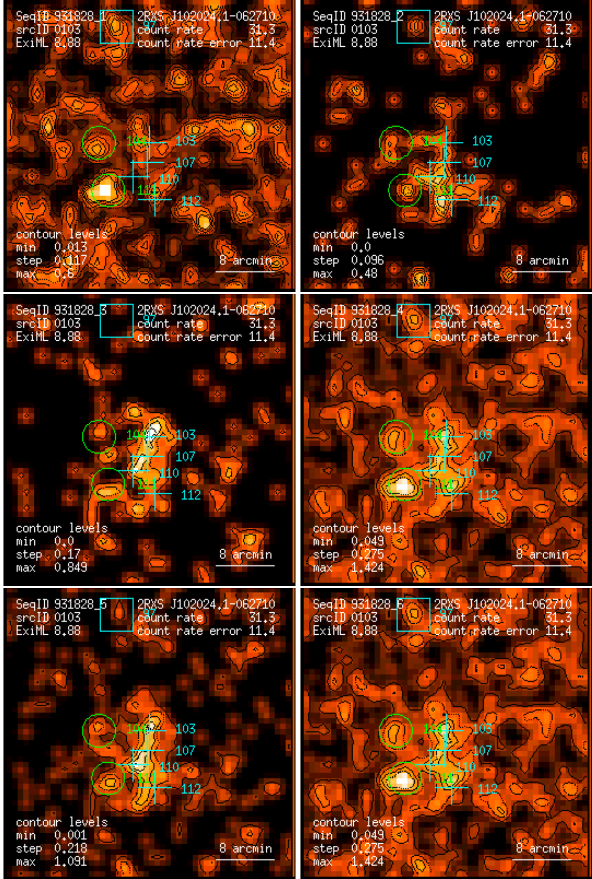
Figure 103: RASS 931828: detection 0103: band rate images, Gaussian filter: (1) PSPC channels 11 – 41, (2) 52 – 90, (3) 91 – 201, (4) 11 – 235, (5) 52 – 201, (6) 11 – 201. Broad band rates in counts/ks. Band rate contour levels in counts/ks/arcmin 2 .
