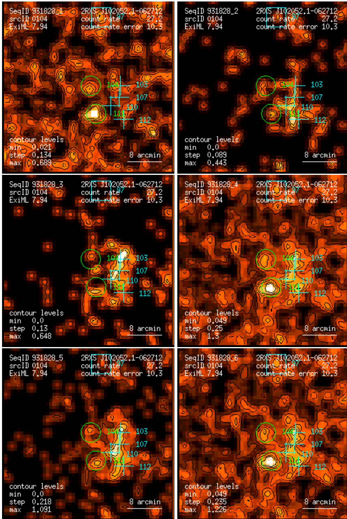
Figure 104: RASS 931828: detection 0104: band rate images, Gaussian filter: (1) PSPC channels 11 – 41, (2) 52 – 90, (3) 91 – 201, (4) 11 – 235, (5) 52 – 201, (6) 11 – 201. Broad band rates in counts/ks. Band rate contour levels in counts/ks/arcmin 2 .
