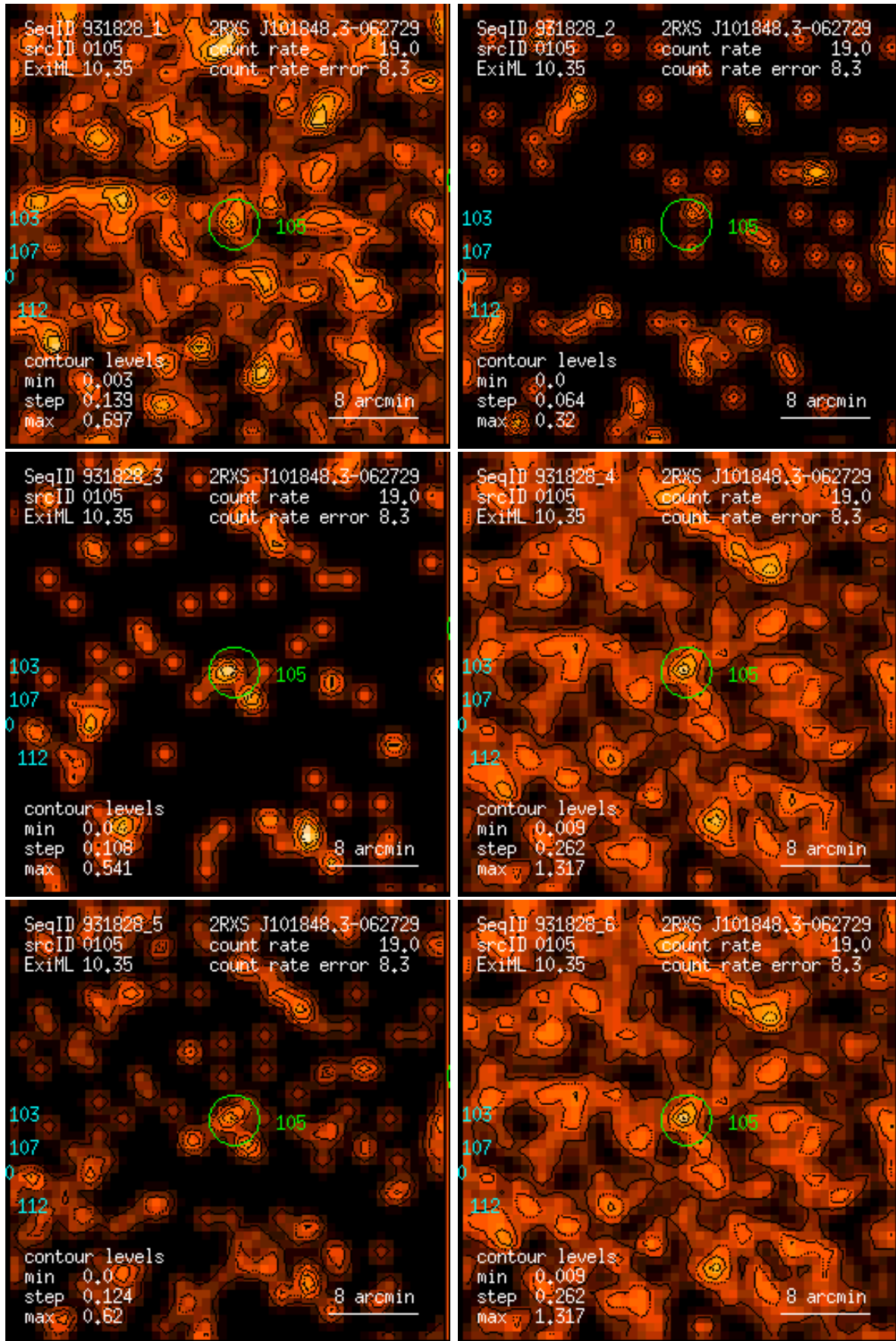
Figure 105: RASS 931828: detection 0105: band rate images, Gaussian filter: (1) PSPC channels 11 – 41, (2) 52 – 90, (3) 91 – 201, (4) 11 – 235, (5) 52 – 201, (6) 11 – 201. Broad band rates in counts/ks. Band rate contour levels in counts/ks/arcmin 2 .
