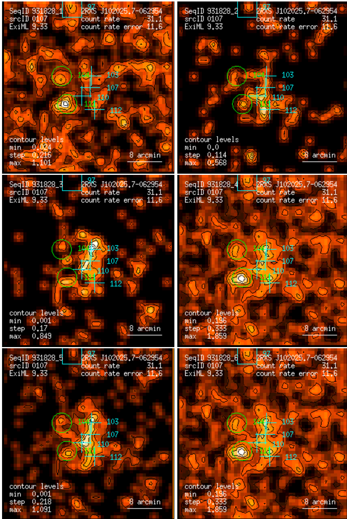
Figure 107: RASS 931828: detection 0107: band rate images, Gaussian filter: (1) PSPC channels 11 – 41, (2) 52 – 90, (3) 91 – 201, (4) 11 – 235, (5) 52 – 201, (6) 11 – 201. Broad band rates in counts/ks. Band rate contour levels in counts/ks/arcmin 2 .
