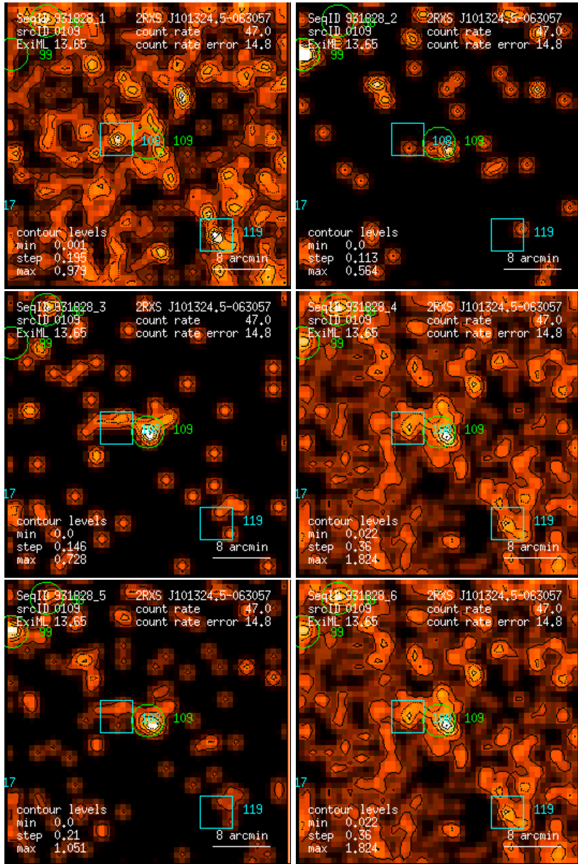
Figure 109: RASS 931828: detection 0109: band rate images, Gaussian filter: (1) PSPC channels 11 – 41, (2) 52 – 90, (3) 91 – 201, (4) 11 – 235, (5) 52 – 201, (6) 11 – 201. Broad band rates in counts/ks. Band rate contour levels in counts/ks/arcmin 2 .
