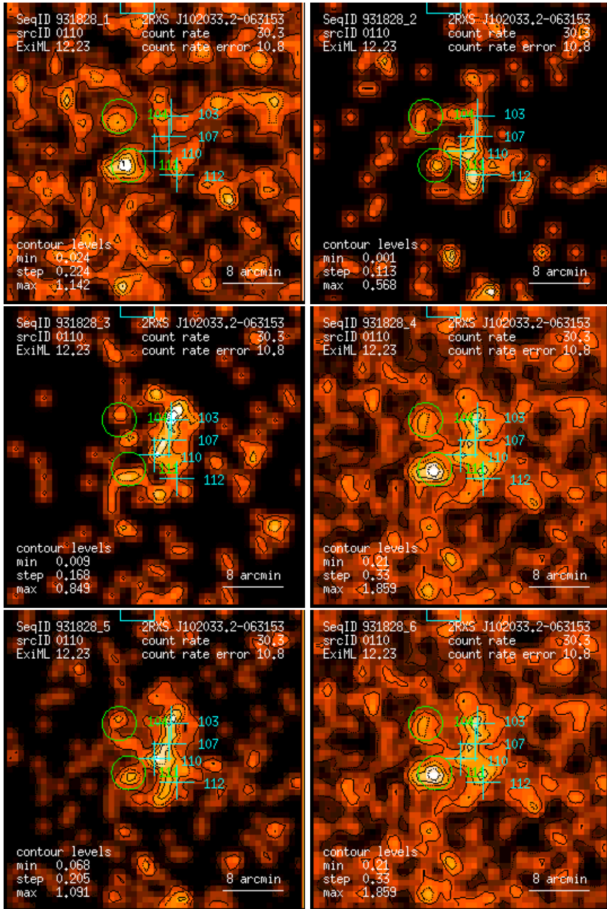
Figure 110: RASS 931828: detection 0110: band rate images, Gaussian filter: (1) PSPC channels 11 – 41, (2) 52 – 90, (3) 91 – 201, (4) 11 – 235, (5) 52 – 201, (6) 11 – 201. Broad band rates in counts/ks. Band rate contour levels in counts/ks/arcmin 2 .
