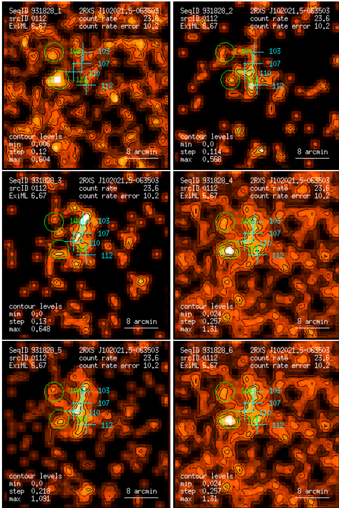
Figure 112: RASS 931828: detection 0112: band rate images, Gaussian filter: (1) PSPC channels 11 – 41, (2) 52 – 90, (3) 91 – 201, (4) 11 – 235, (5) 52 – 201, (6) 11 – 201. Broad band rates in counts/ks. Band rate contour levels in counts/ks/arcmin 2 .
