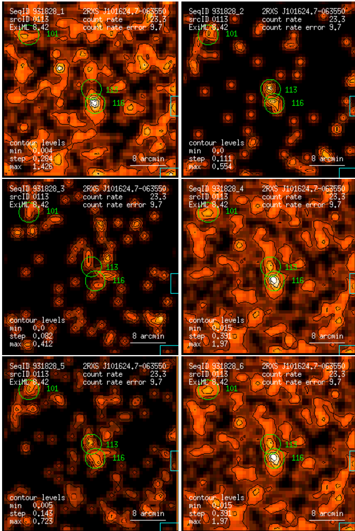
Figure 113: RASS 931828: detection 0113: band rate images, Gaussian filter: (1) PSPC channels 11 – 41, (2) 52 – 90, (3) 91 – 201, (4) 11 – 235, (5) 52 – 201, (6) 11 – 201. Broad band rates in counts/ks. Band rate contour levels in counts/ks/arcmin 2 .
