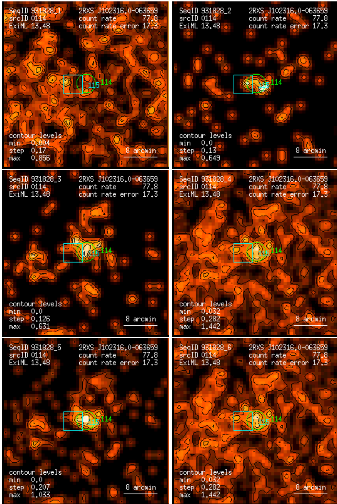
Figure 114: RASS 931828: detection 0114: band rate images, Gaussian filter: (1) PSPC channels 11 – 41, (2) 52 – 90, (3) 91 – 201, (4) 11 – 235, (5) 52 – 201, (6) 11 – 201. Broad band rates in counts/ks. Band rate contour levels in counts/ks/arcmin 2 .
