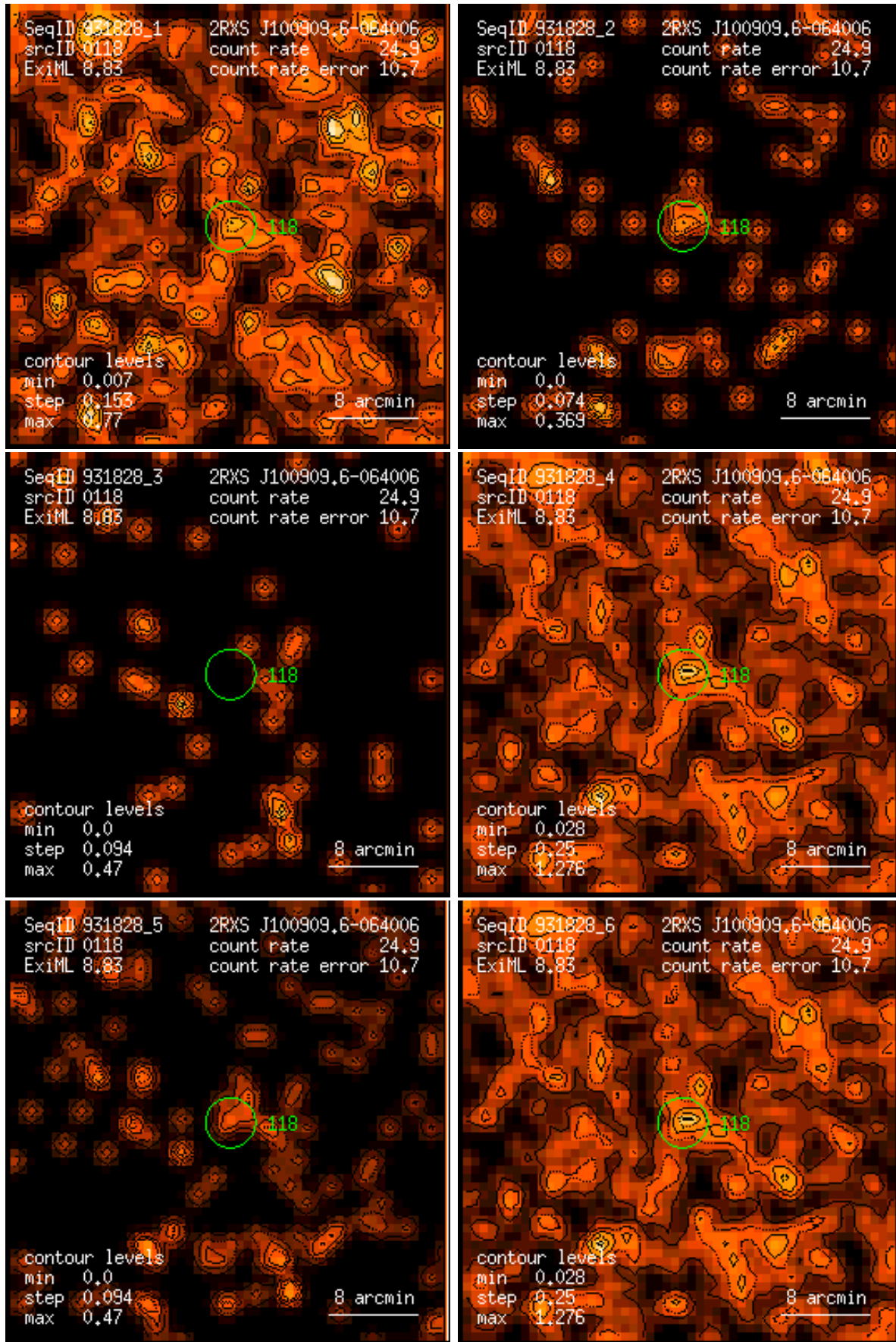
Figure 118: RASS 931828: detection 0118: band rate images, Gaussian filter: (1) PSPC channels 11 – 41, (2) 52 – 90, (3) 91 – 201, (4) 11 – 235, (5) 52 – 201, (6) 11 – 201. Broad band rates in counts/ks. Band rate contour levels in counts/ks/arcmin 2 .
