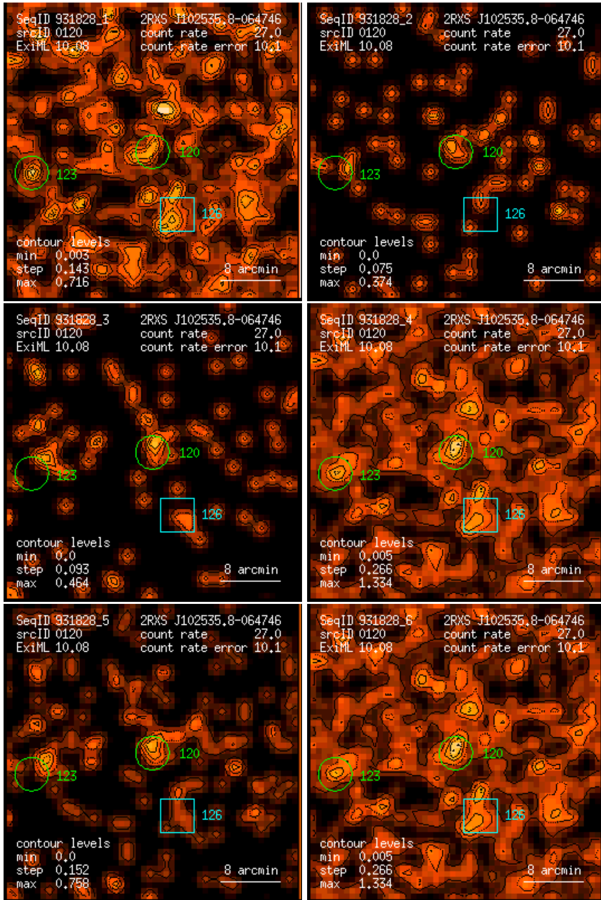
Figure 120: RASS 931828: detection 0120: band rate images, Gaussian filter: (1) PSPC channels 11 – 41, (2) 52 – 90, (3) 91 – 201, (4) 11 – 235, (5) 52 – 201, (6) 11 – 201. Broad band rates in counts/ks. Band rate contour levels in counts/ks/arcmin 2 .
