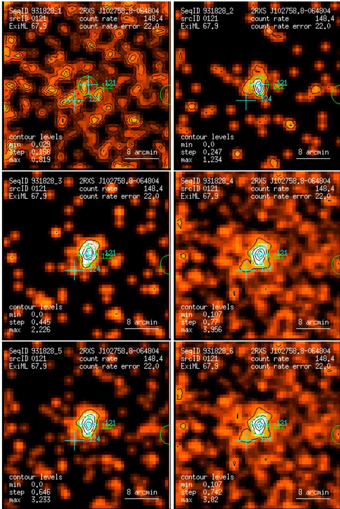
Figure 121: RASS 931828: detection 0121: band rate images, Gaussian filter: (1) PSPC channels 11 – 41, (2) 52 – 90, (3) 91 – 201, (4) 11 – 235, (5) 52 – 201, (6) 11 – 201. Broad band rates in counts/ks. Band rate contour levels in counts/ks/arcmin 2 .
