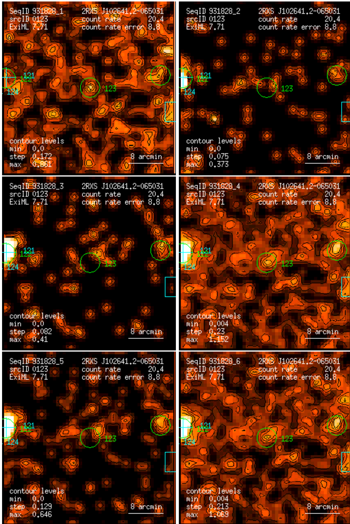
Figure 123: RASS 931828: detection 0123: band rate images, Gaussian filter: (1) PSPC channels 11 – 41, (2) 52 – 90, (3) 91 – 201, (4) 11 – 235, (5) 52 – 201, (6) 11 – 201. Broad band rates in counts/ks. Band rate contour levels in counts/ks/arcmin 2 .
