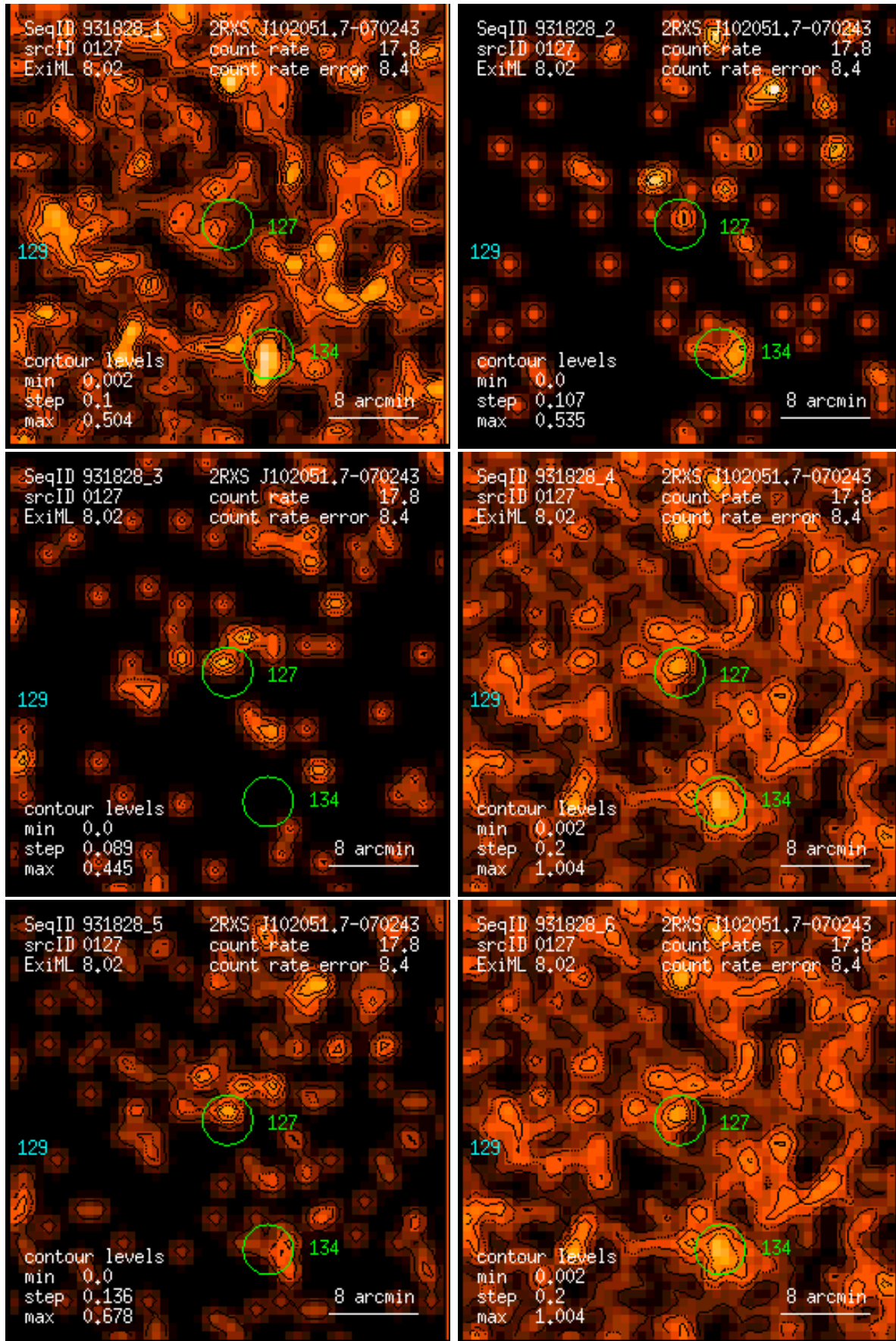
Figure 127: RASS 931828: detection 0127: band rate images, Gaussian filter: (1) PSPC channels 11 – 41, (2) 52 – 90, (3) 91 – 201, (4) 11 – 235, (5) 52 – 201, (6) 11 – 201. Broad band rates in counts/ks. Band rate contour levels in counts/ks/arcmin 2 .
