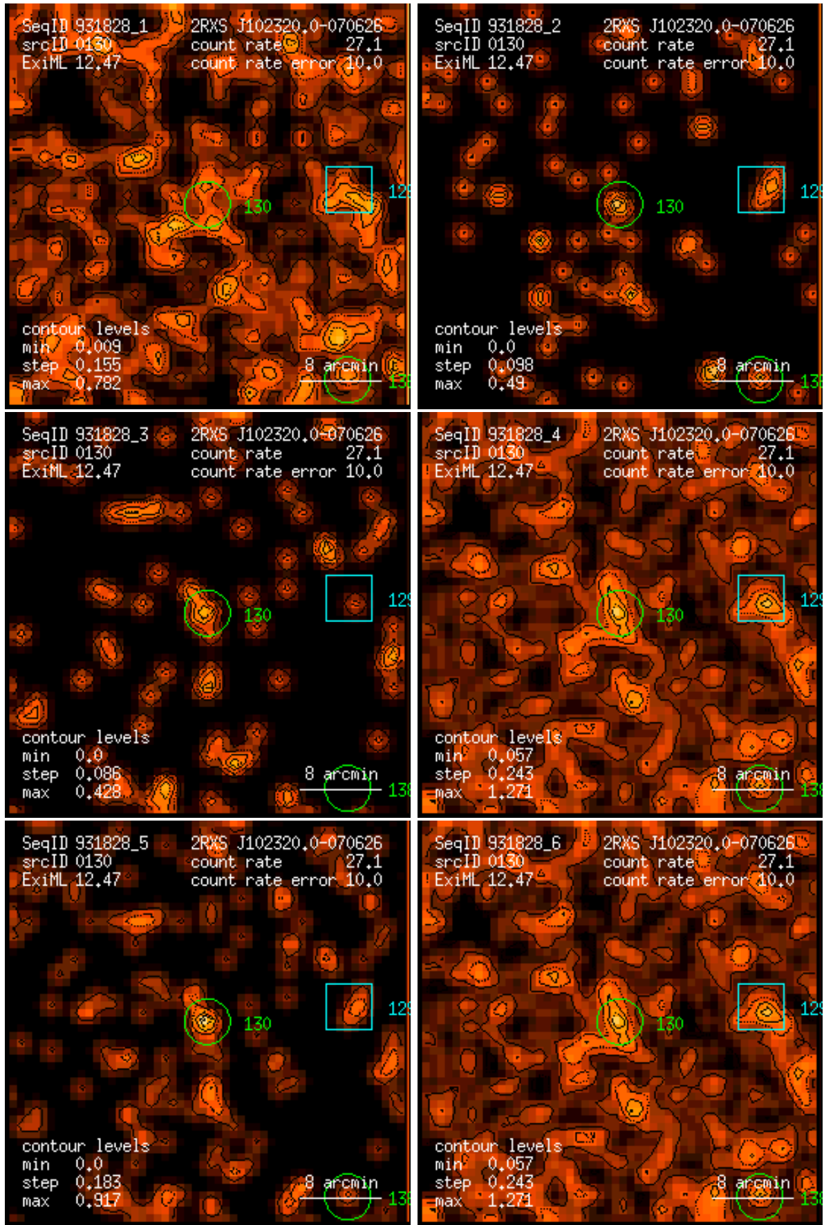
Figure 130: RASS 931828: detection 0130: band rate images, Gaussian filter: (1) PSPC channels 11 – 41, (2) 52 – 90, (3) 91 – 201, (4) 11 – 235, (5) 52 – 201, (6) 11 – 201. Broad band rates in counts/ks. Band rate contour levels in counts/ks/arcmin 2 .
