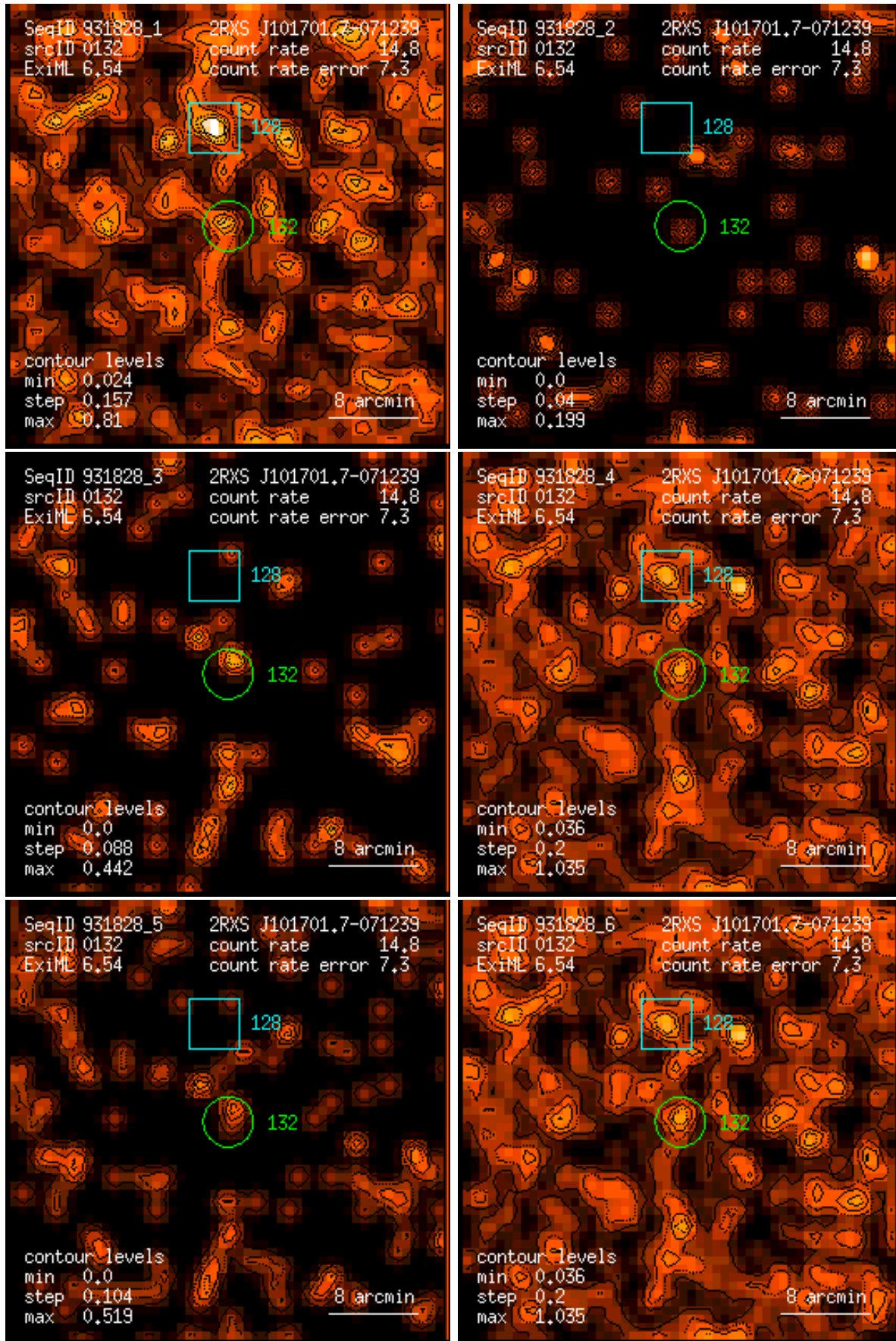
Figure 132: RASS 931828: detection 0132: band rate images, Gaussian filter: (1) PSPC channels 11 – 41, (2) 52 – 90, (3) 91 – 201, (4) 11 – 235, (5) 52 – 201, (6) 11 – 201. Broad band rates in counts/ks. Band rate contour levels in counts/ks/arcmin 2 .
