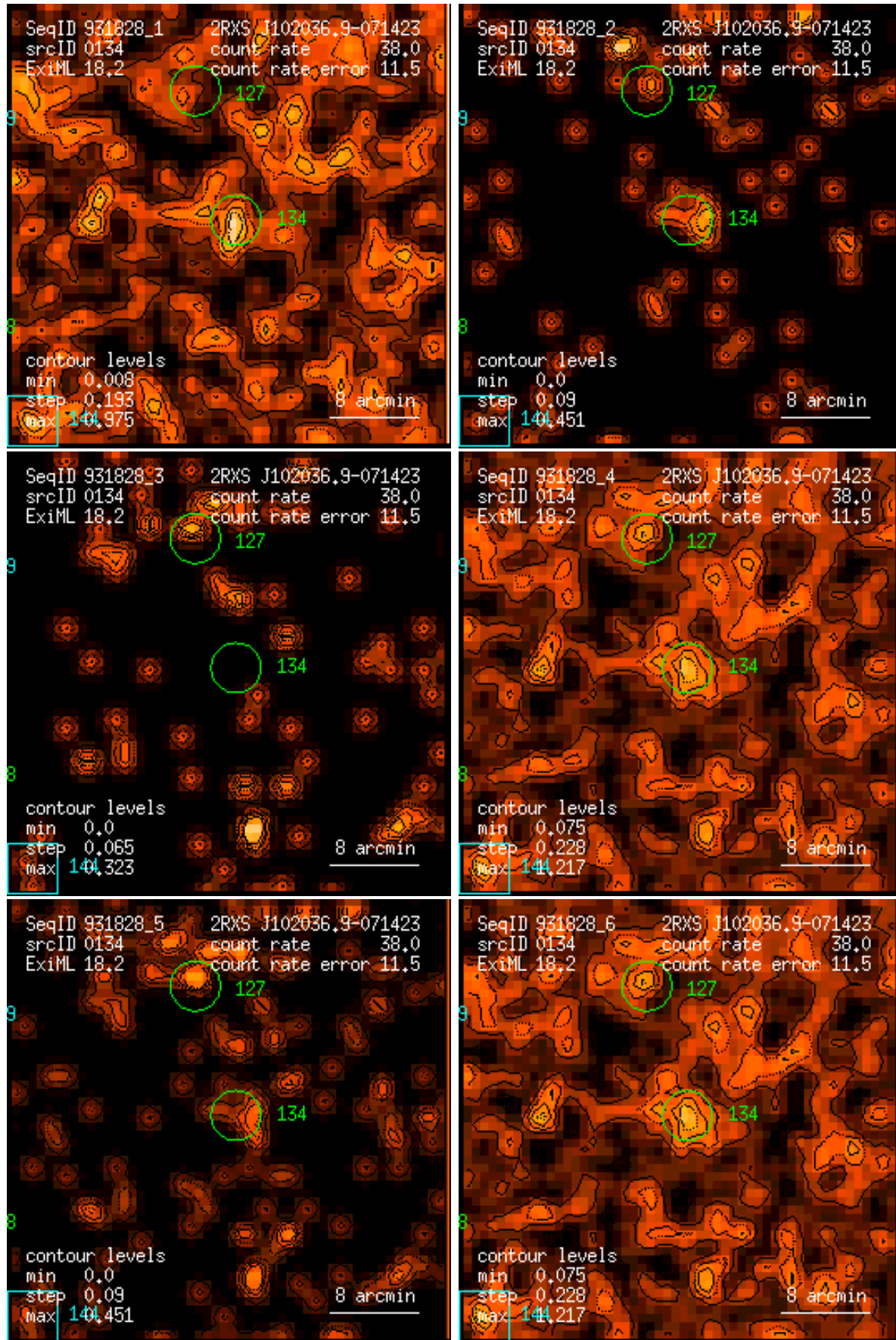
Figure 134: RASS 931828: detection 0134: band rate images, Gaussian filter: (1) PSPC channels 11 – 41, (2) 52 – 90, (3) 91 – 201, (4) 11 – 235, (5) 52 – 201, (6) 11 – 201. Broad band rates in counts/ks. Band rate contour levels in counts/ks/arcmin 2 .
