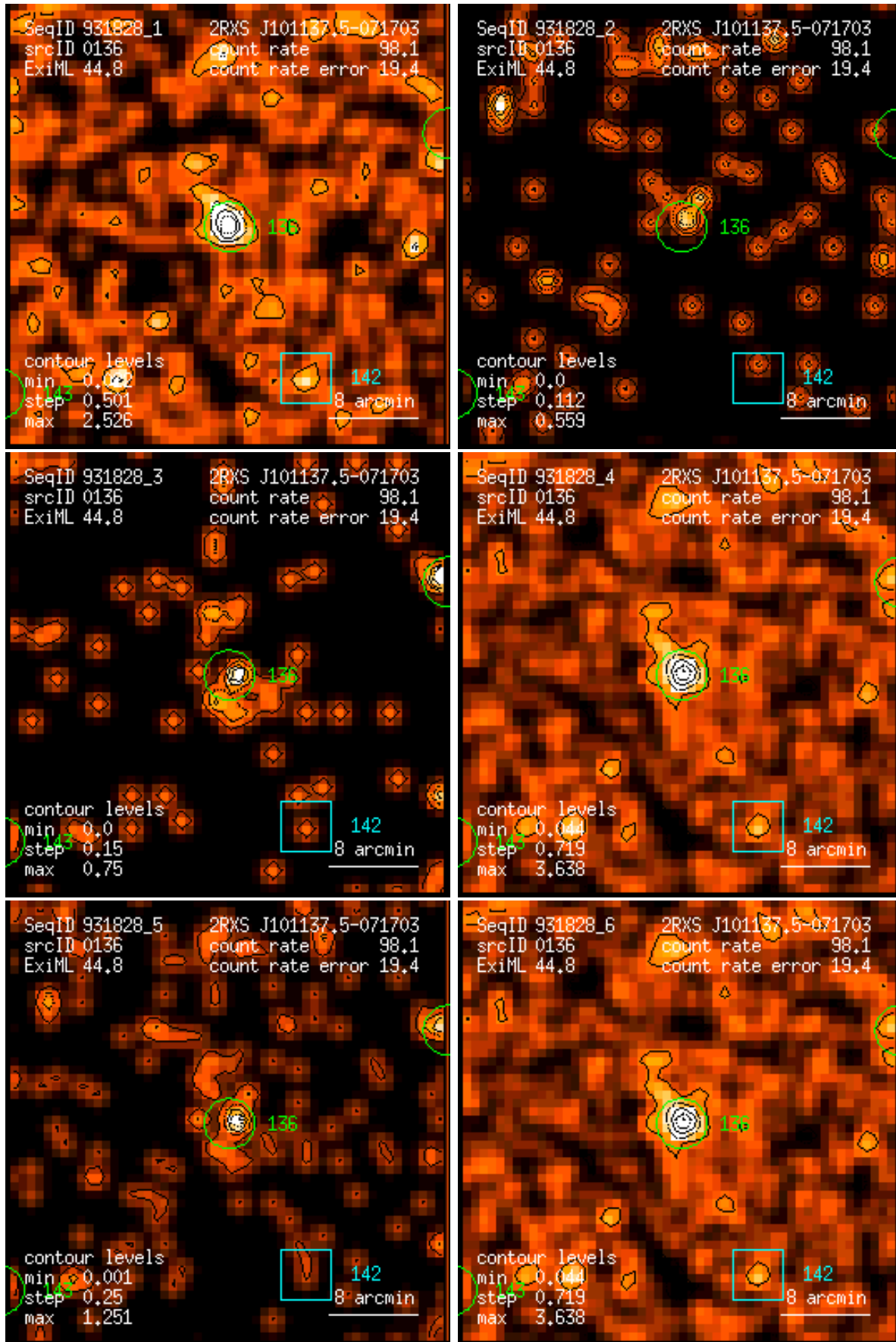
Figure 136: RASS 931828: detection 0136: band rate images, Gaussian filter: (1) PSPC channels 11 – 41, (2) 52 – 90, (3) 91 – 201, (4) 11 – 235, (5) 52 – 201, (6) 11 – 201. Broad band rates in counts/ks. Band rate contour levels in counts/ks/arcmin 2 .
