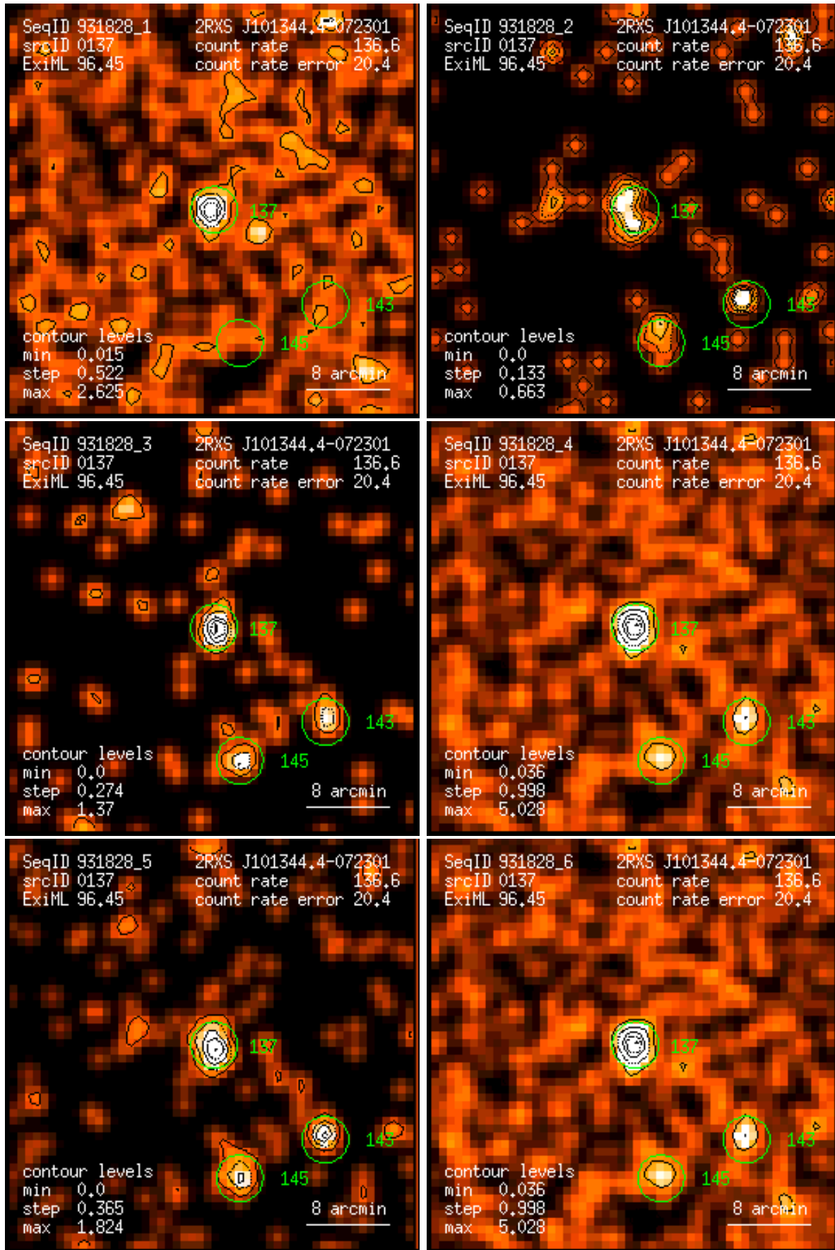
Figure 137: RASS 931828: detection 0137: band rate images, Gaussian filter: (1) PSPC channels 11 – 41, (2) 52 – 90, (3) 91 – 201, (4) 11 – 235, (5) 52 – 201, (6) 11 – 201. Broad band rates in counts/ks. Band rate contour levels in counts/ks/arcmin 2 .
