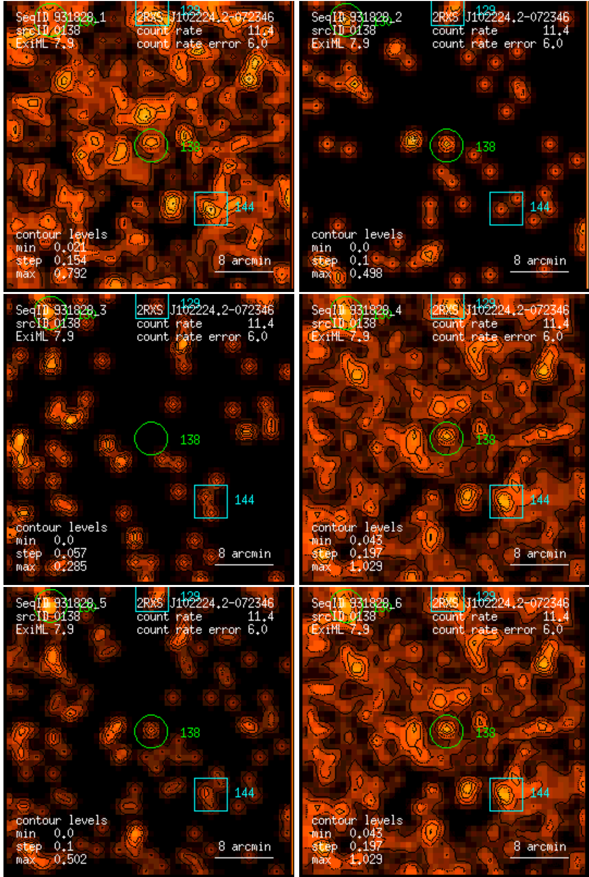
Figure 138: RASS 931828: detection 0138: band rate images, Gaussian filter: (1) PSPC channels 11 – 41, (2) 52 – 90, (3) 91 – 201, (4) 11 – 235, (5) 52 – 201, (6) 11 – 201. Broad band rates in counts/ks. Band rate contour levels in counts/ks/arcmin 2 .
