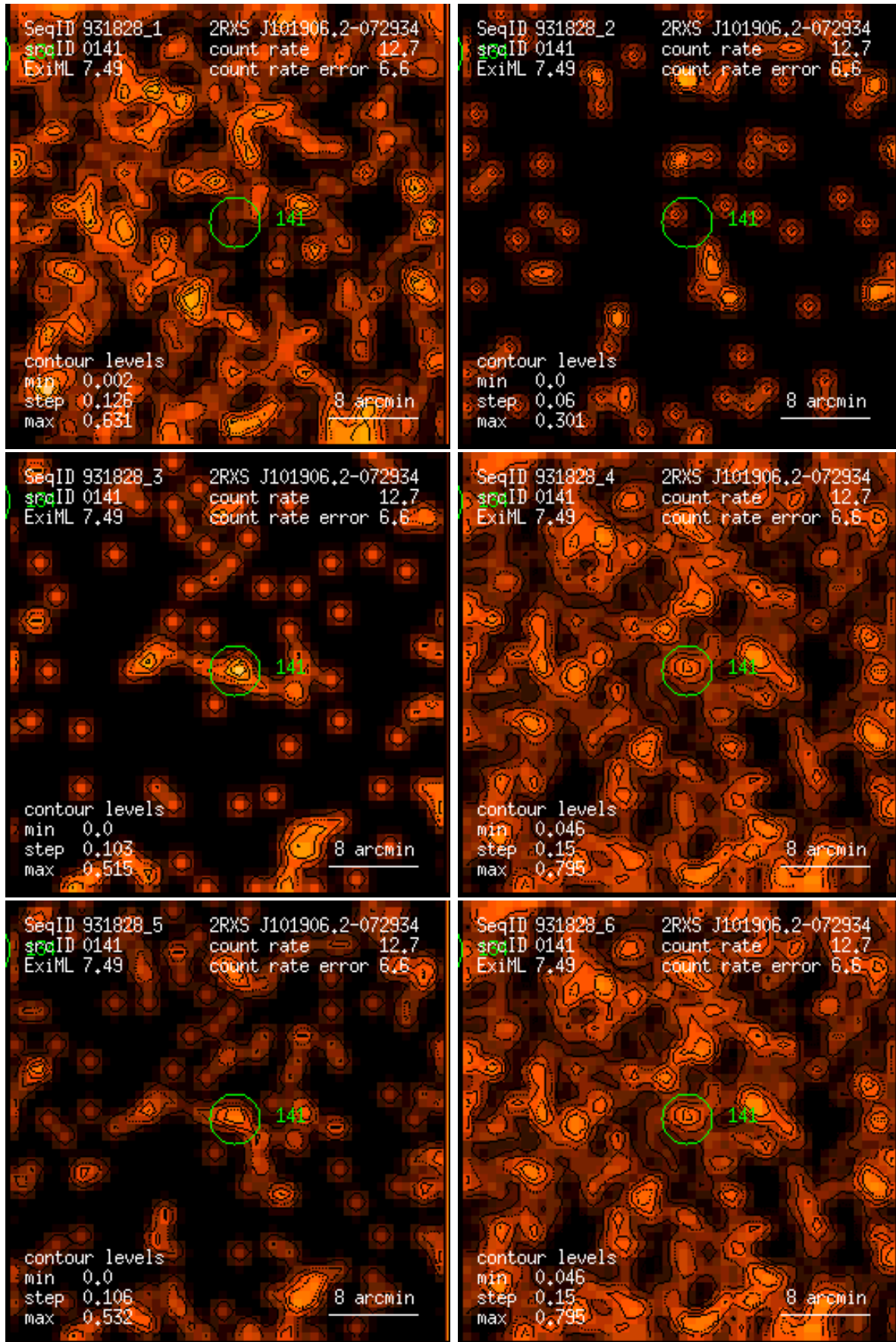
Figure 141: RASS 931828: detection 0141: band rate images, Gaussian filter: (1) PSPC channels 11 – 41, (2) 52 – 90, (3) 91 – 201, (4) 11 – 235, (5) 52 – 201, (6) 11 – 201. Broad band rates in counts/ks. Band rate contour levels in counts/ks/arcmin 2 .
