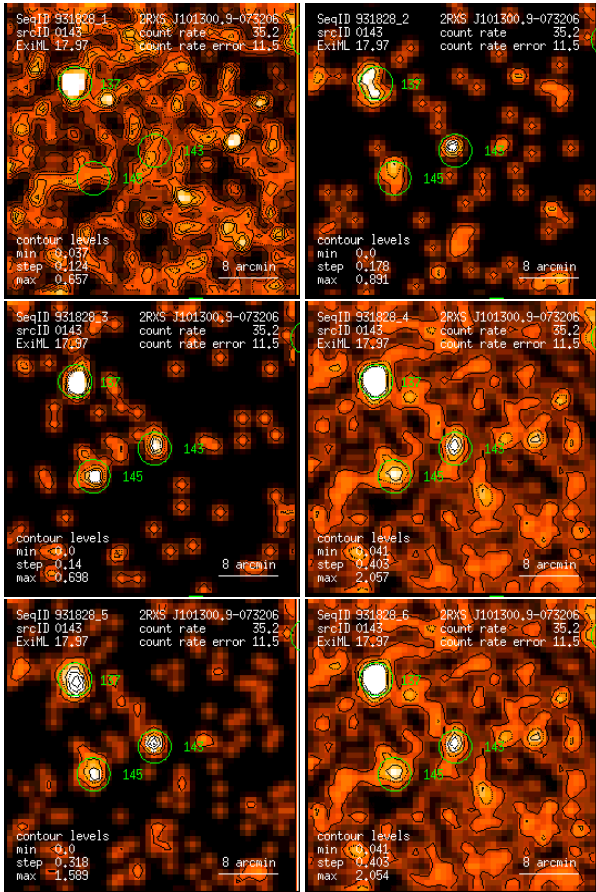
Figure 143: RASS 931828: detection 0143: band rate images, Gaussian filter: (1) PSPC channels 11 – 41, (2) 52 – 90, (3) 91 – 201, (4) 11 – 235, (5) 52 – 201, (6) 11 – 201. Broad band rates in counts/ks. Band rate contour levels in counts/ks/arcmin 2 .
