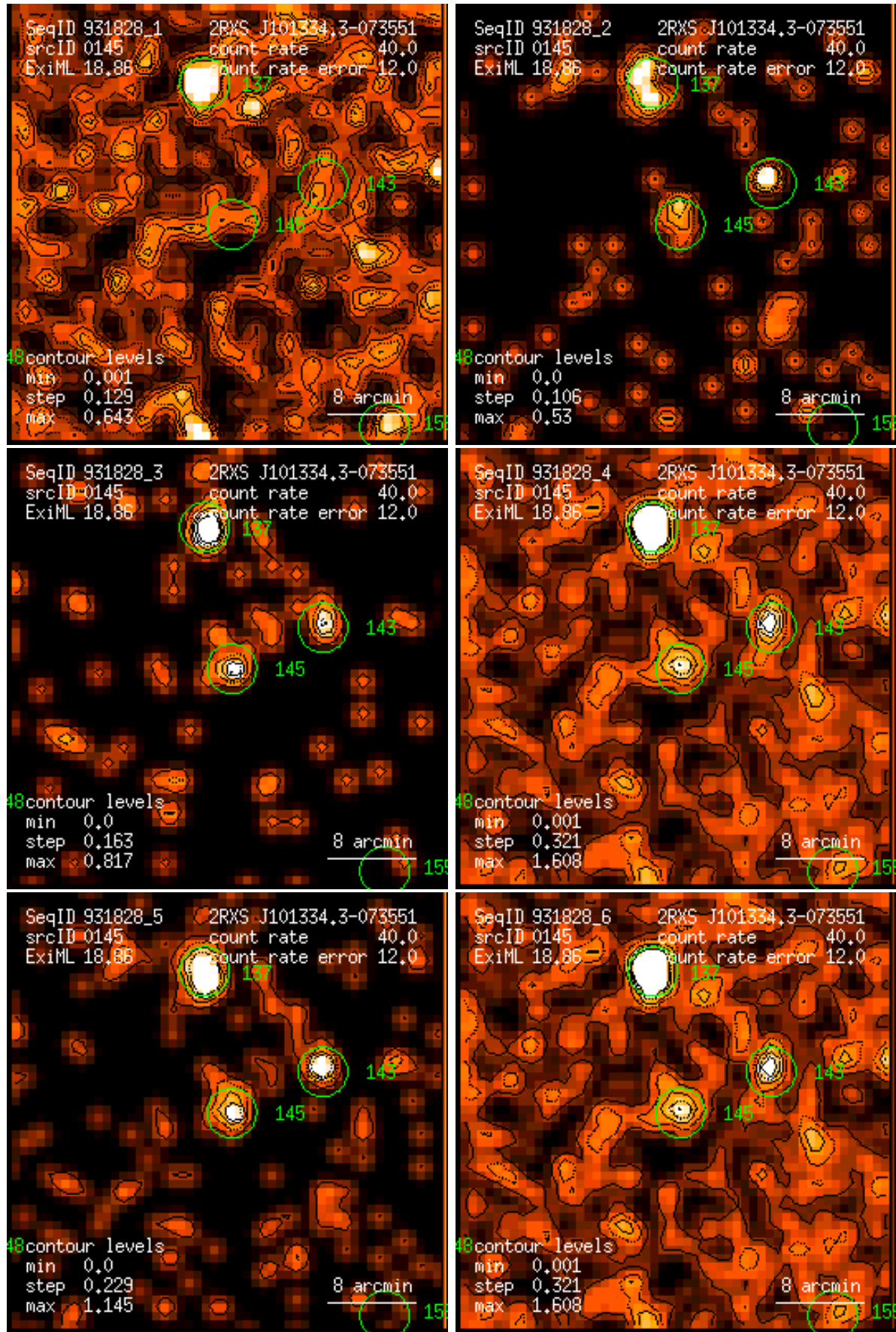
Figure 145: RASS 931828: detection 0145: band rate images, Gaussian filter: (1) PSPC channels 11 – 41, (2) 52 – 90, (3) 91 – 201, (4) 11 – 235, (5) 52 – 201, (6) 11 – 201. Broad band rates in counts/ks. Band rate contour levels in counts/ks/arcmin 2 .
