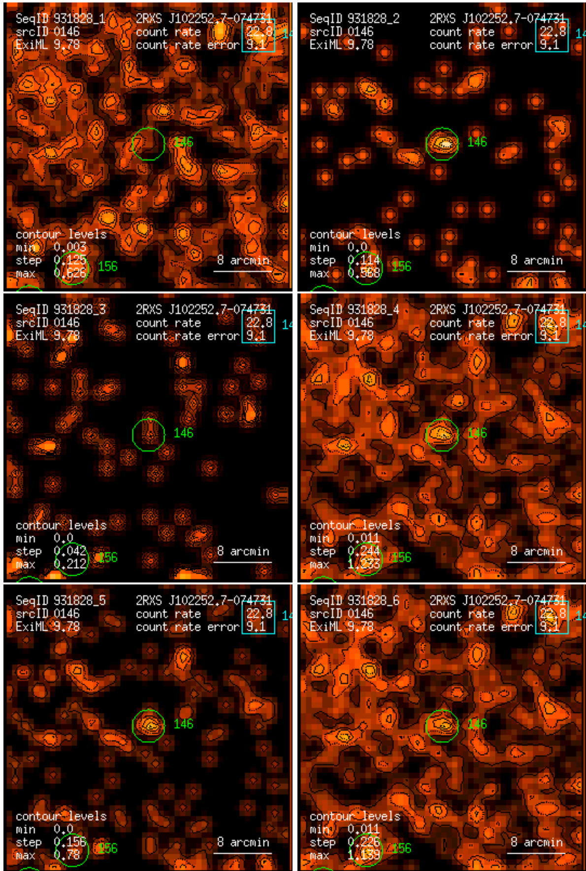
Figure 146: RASS 931828: detection 0146: band rate images, Gaussian filter: (1) PSPC channels 11 – 41, (2) 52 – 90, (3) 91 – 201, (4) 11 – 235, (5) 52 – 201, (6) 11 – 201. Broad band rates in counts/ks. Band rate contour levels in counts/ks/arcmin 2 .
