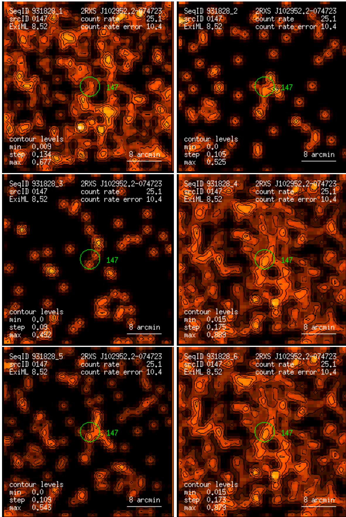
Figure 147: RASS 931828: detection 0147: band rate images, Gaussian filter: (1) PSPC channels 11 – 41, (2) 52 – 90, (3) 91 – 201, (4) 11 – 235, (5) 52 – 201, (6) 11 – 201. Broad band rates in counts/ks. Band rate contour levels in counts/ks/arcmin 2 .
