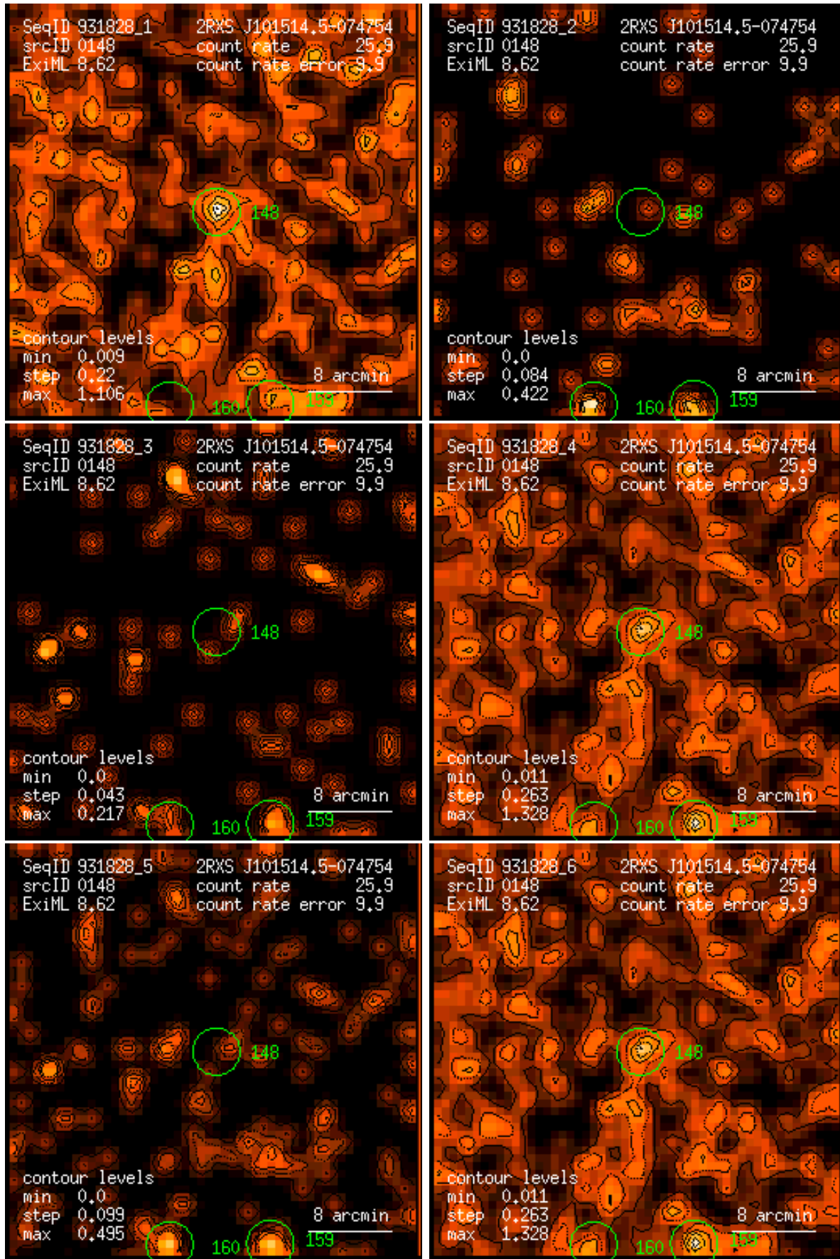
Figure 148: RASS 931828: detection 0148: band rate images, Gaussian filter: (1) PSPC channels 11 – 41, (2) 52 – 90, (3) 91 – 201, (4) 11 – 235, (5) 52 – 201, (6) 11 – 201. Broad band rates in counts/ks. Band rate contour levels in counts/ks/arcmin 2 .
