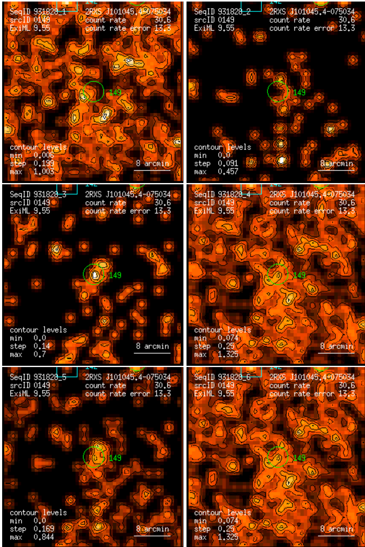
Figure 149: RASS 931828: detection 0149: band rate images, Gaussian filter: (1) PSPC channels 11 – 41, (2) 52 – 90, (3) 91 – 201, (4) 11 – 235, (5) 52 – 201, (6) 11 – 201. Broad band rates in counts/ks. Band rate contour levels in counts/ks/arcmin 2 .
