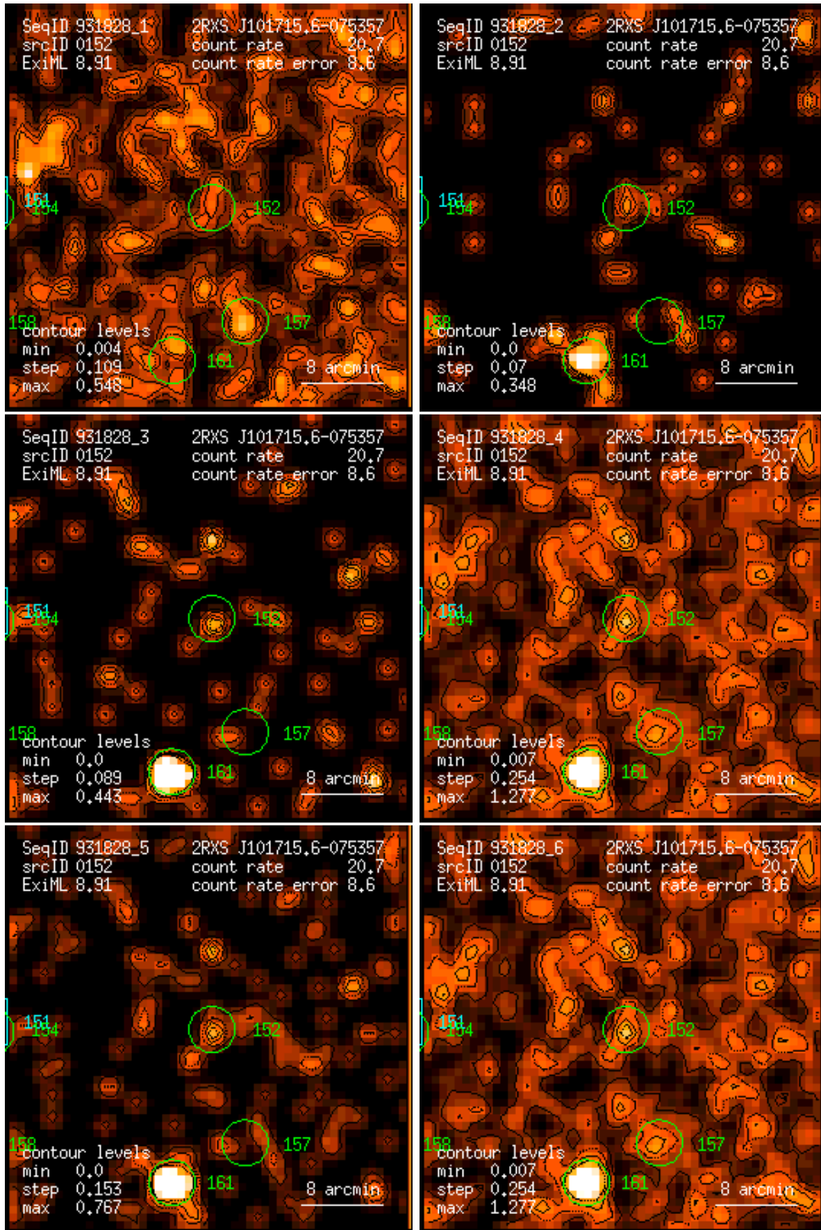
Figure 152: RASS 931828: detection 0152: band rate images, Gaussian filter: (1) PSPC channels 11 – 41, (2) 52 – 90, (3) 91 – 201, (4) 11 – 235, (5) 52 – 201, (6) 11 – 201. Broad band rates in counts/ks. Band rate contour levels in counts/ks/arcmin 2 .
