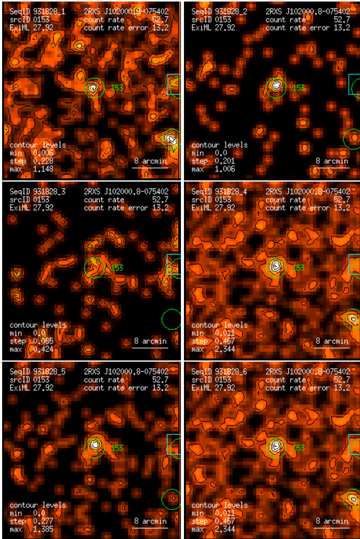
Figure 153: RASS 931828: detection 0153: band rate images, Gaussian filter: (1) PSPC channels 11 – 41, (2) 52 – 90, (3) 91 – 201, (4) 11 – 235, (5) 52 – 201, (6) 11 – 201. Broad band rates in counts/ks. Band rate contour levels in counts/ks/arcmin 2 .
