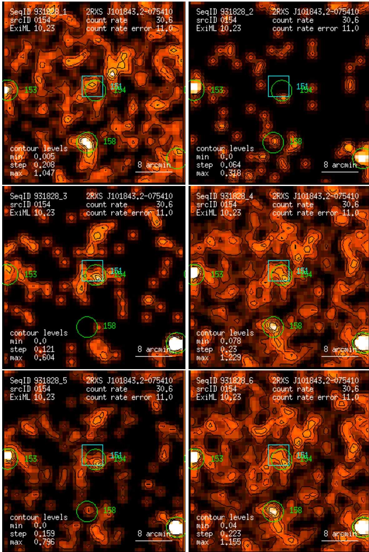
Figure 154: RASS 931828: detection 0154: band rate images, Gaussian filter: (1) PSPC channels 11 – 41, (2) 52 – 90, (3) 91 – 201, (4) 11 – 235, (5) 52 – 201, (6) 11 – 201. Broad band rates in counts/ks. Band rate contour levels in counts/ks/arcmin 2 .
