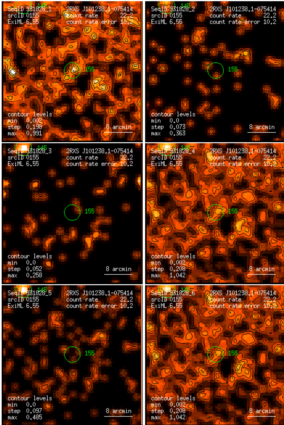
Figure 155: RASS 931828: detection 0155: band rate images, Gaussian filter: (1) PSPC channels 11 – 41, (2) 52 – 90, (3) 91 – 201, (4) 11 – 235, (5) 52 – 201, (6) 11 – 201. Broad band rates in counts/ks. Band rate contour levels in counts/ks/arcmin 2 .
