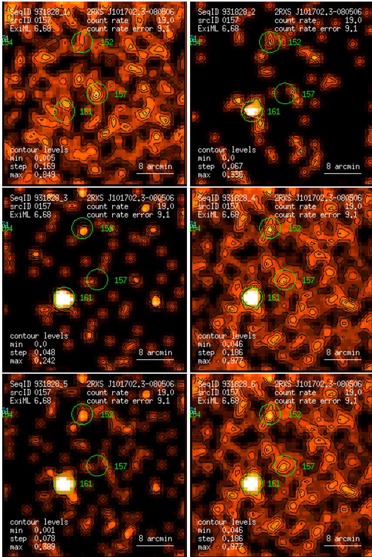
Figure 157: RASS 931828: detection 0157: band rate images, Gaussian filter: (1) PSPC channels 11 – 41, (2) 52 – 90, (3) 91 – 201, (4) 11 – 235, (5) 52 – 201, (6) 11 – 201. Broad band rates in counts/ks. Band rate contour levels in counts/ks/arcmin 2 .
