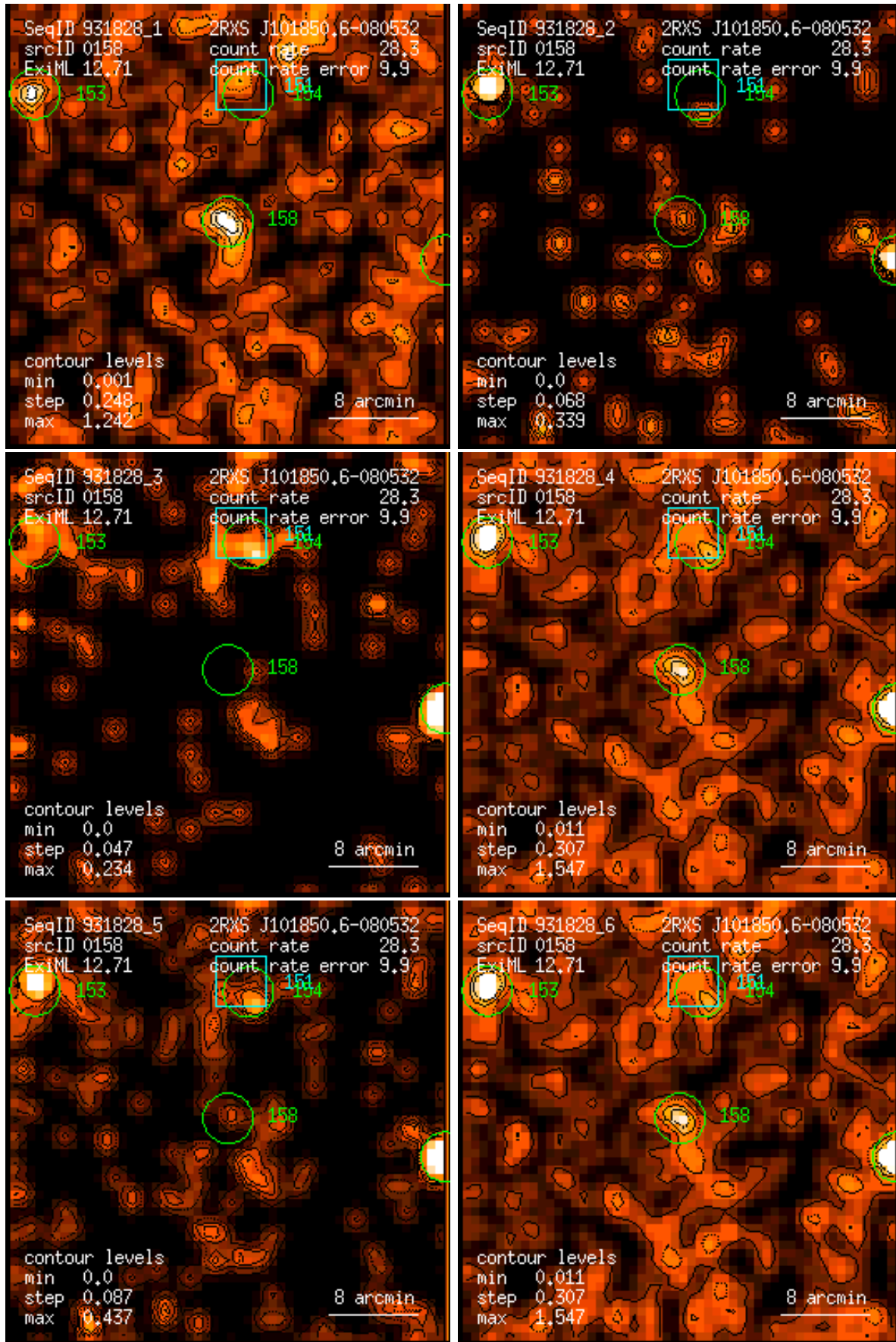
Figure 158: RASS 931828: detection 0158: band rate images, Gaussian filter: (1) PSPC channels 11 – 41, (2) 52 – 90, (3) 91 – 201, (4) 11 – 235, (5) 52 – 201, (6) 11 – 201. Broad band rates in counts/ks. Band rate contour levels in counts/ks/arcmin 2 .
