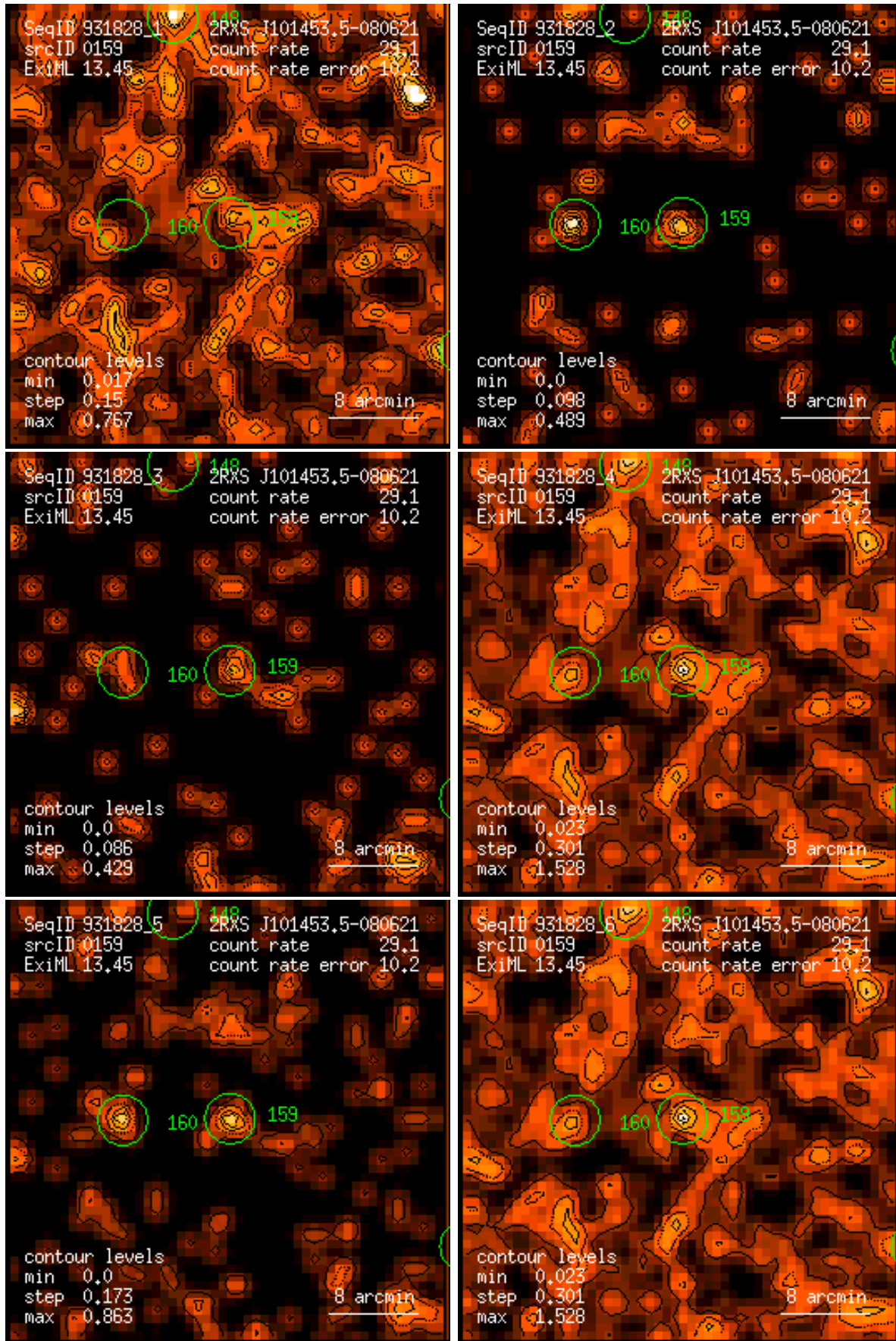
Figure 159: RASS 931828: detection 0159: band rate images, Gaussian filter: (1) PSPC channels 11 – 41, (2) 52 – 90, (3) 91 – 201, (4) 11 – 235, (5) 52 – 201, (6) 11 – 201. Broad band rates in counts/ks. Band rate contour levels in counts/ks/arcmin 2 .
