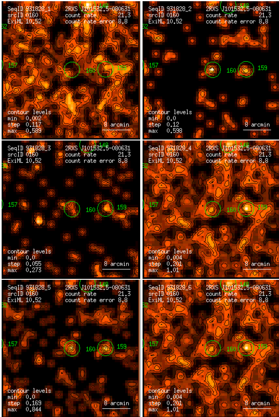
Figure 160: RASS 931828: detection 0160: band rate images, Gaussian filter: (1) PSPC channels 11 – 41, (2) 52 – 90, (3) 91 – 201, (4) 11 – 235, (5) 52 – 201, (6) 11 – 201. Broad band rates in counts/ks. Band rate contour levels in counts/ks/arcmin 2 .
