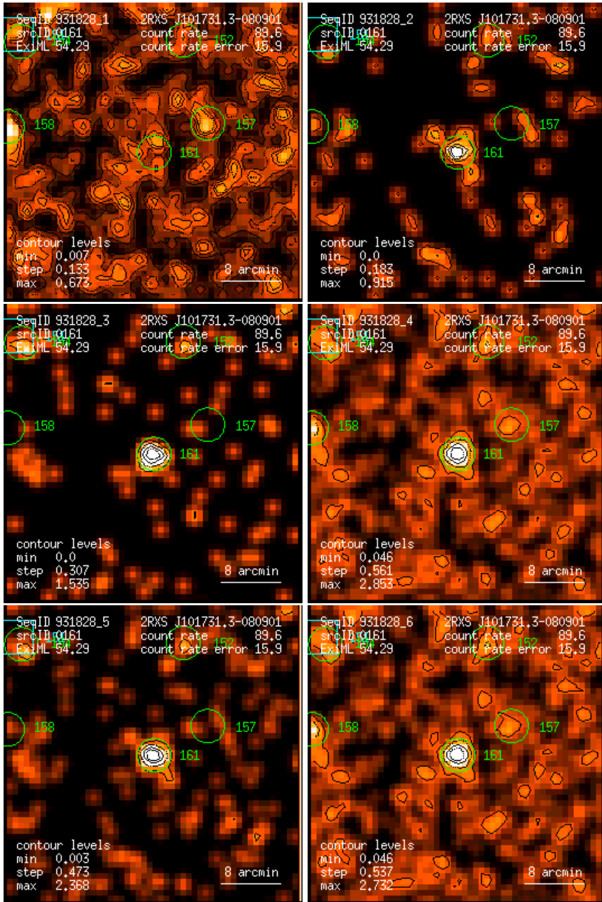
Figure 161: RASS 931828: detection 0161: band rate images, Gaussian filter: (1) PSPC channels 11 – 41, (2) 52 – 90, (3) 91 – 201, (4) 11 – 235, (5) 52 – 201, (6) 11 – 201. Broad band rates in counts/ks. Band rate contour levels in counts/ks/arcmin 2 .
