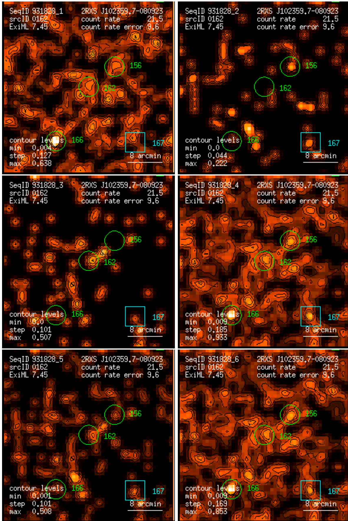
Figure 162: RASS 931828: detection 0162: band rate images, Gaussian filter: (1) PSPC channels 11 – 41, (2) 52 – 90, (3) 91 – 201, (4) 11 – 235, (5) 52 – 201, (6) 11 – 201. Broad band rates in counts/ks. Band rate contour levels in counts/ks/arcmin 2 .
