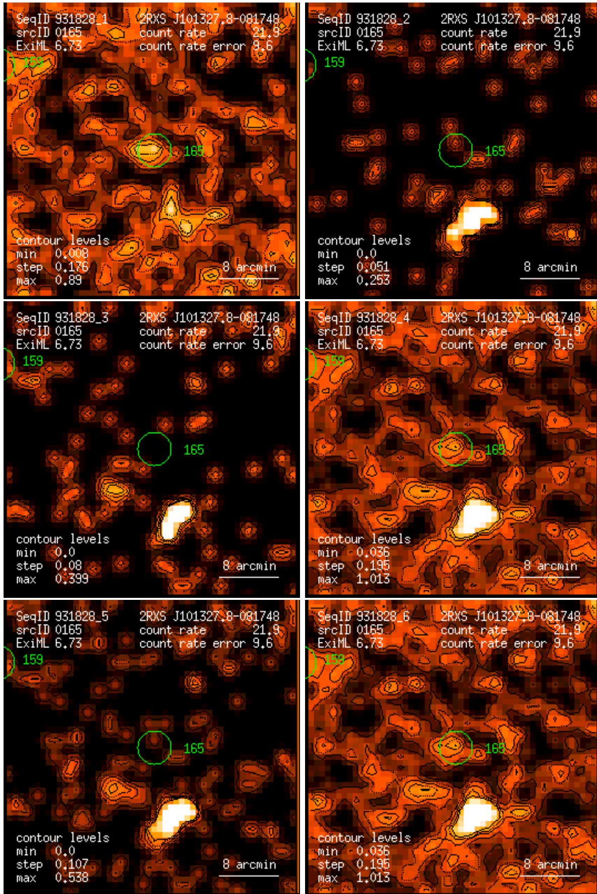
Figure 165: RASS 931828: detection 0165: band rate images, Gaussian filter: (1) PSPC channels 11 – 41, (2) 52 – 90, (3) 91 – 201, (4) 11 – 235, (5) 52 – 201, (6) 11 – 201. Broad band rates in counts/ks. Band rate contour levels in counts/ks/arcmin 2 .
