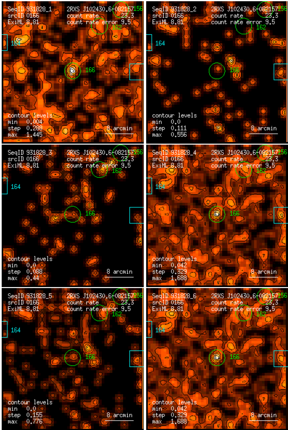
Figure 166: RASS 931828: detection 0166: band rate images, Gaussian filter: (1) PSPC channels 11 – 41, (2) 52 – 90, (3) 91 – 201, (4) 11 – 235, (5) 52 – 201, (6) 11 – 201. Broad band rates in counts/ks. Band rate contour levels in counts/ks/arcmin 2 .
