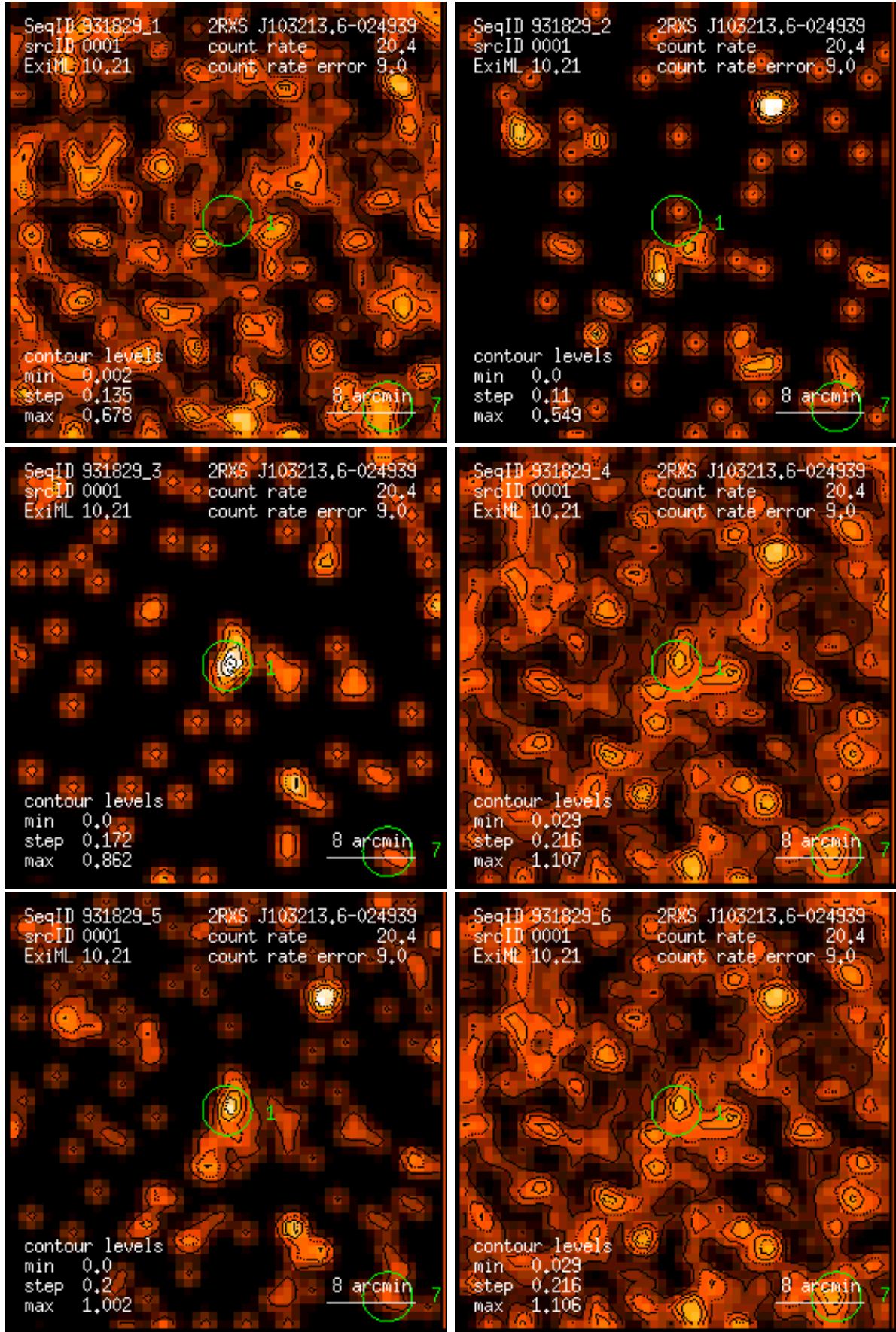
Figure 1: RASS 931829: detection 0001: band rate images, Gaussian filter: (1) PSPC channels 11 – 41, (2) 52 – 90, (3) 91 – 201, (4) 11 – 235, (5) 52 – 201, (6) 11 – 201. Broad band rates in counts/ks. Band rate contour levels in counts/ks/arcmin 2 .
