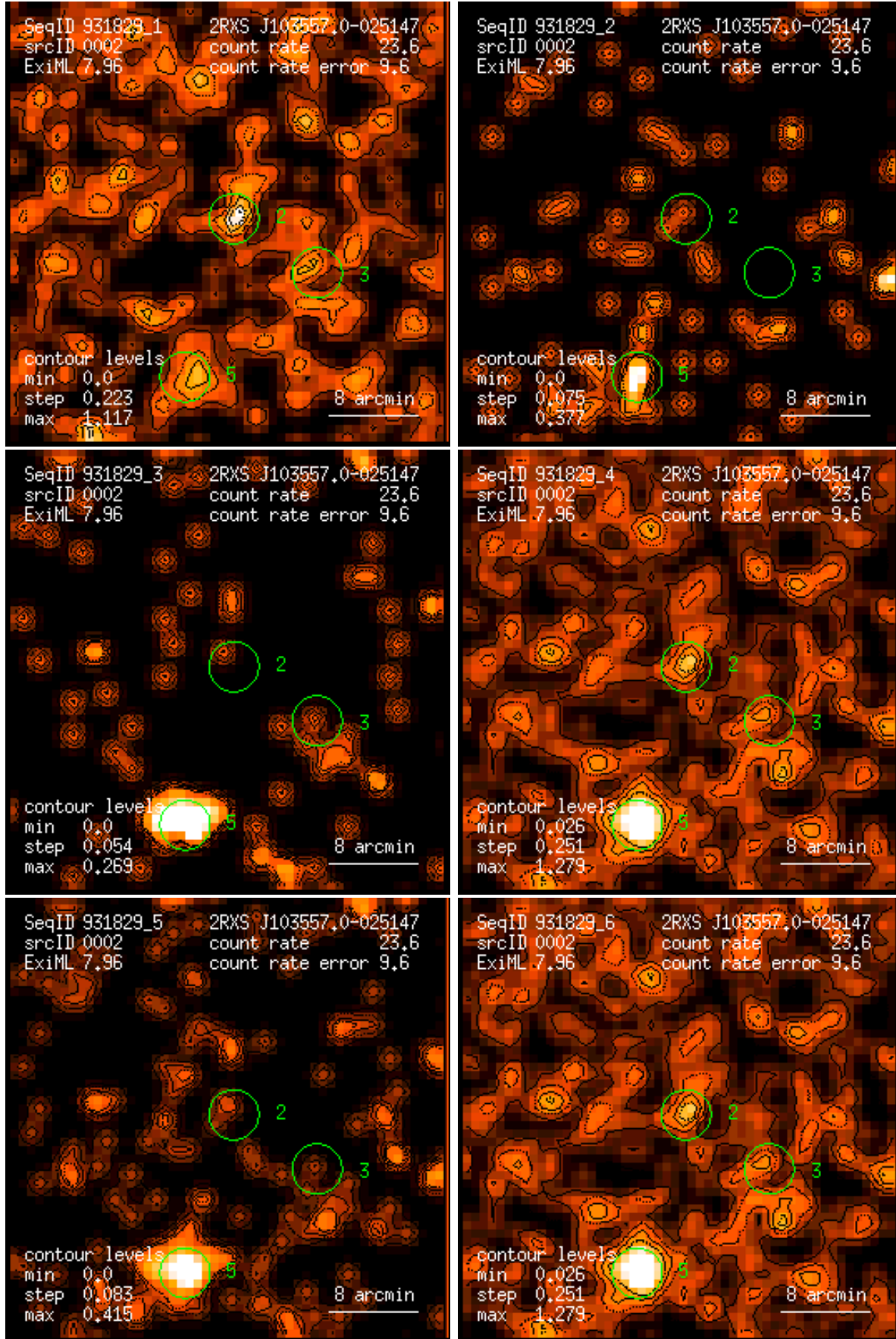
Figure 2: RASS 931829: detection 0002: band rate images, Gaussian filter: (1) PSPC channels 11 – 41, (2) 52 – 90, (3) 91 – 201, (4) 11 – 235, (5) 52 – 201, (6) 11 – 201. Broad band rates in counts/ks. Band rate contour levels in counts/ks/arcmin 2 .
