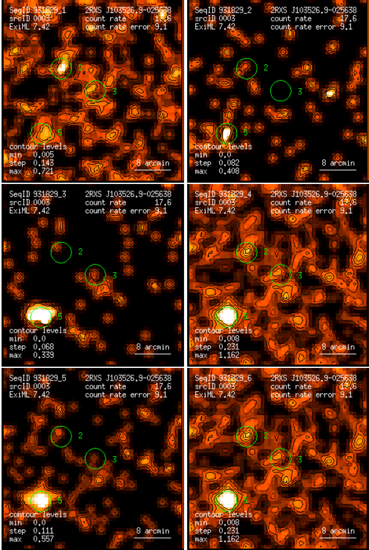
Figure 3: RASS 931829: detection 0003: band rate images, Gaussian filter: (1) PSPC channels 11 – 41, (2) 52 – 90, (3) 91 – 201, (4) 11 – 235, (5) 52 – 201, (6) 11 – 201. Broad band rates in counts/ks. Band rate contour levels in counts/ks/arcmin 2 .
