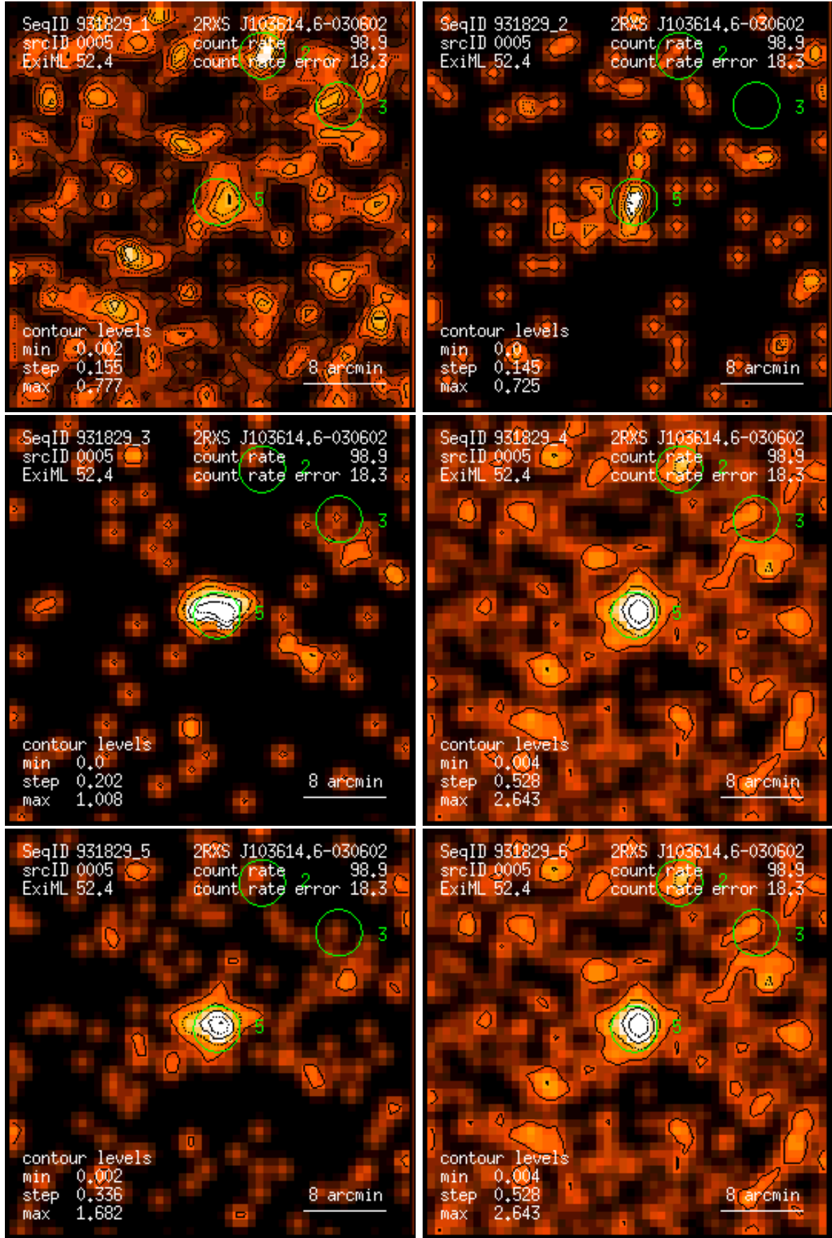
Figure 5: RASS 931829: detection 0005: band rate images, Gaussian filter: (1) PSPC channels 11 – 41, (2) 52 – 90, (3) 91 – 201, (4) 11 – 235, (5) 52 – 201, (6) 11 – 201. Broad band rates in counts/ks. Band rate contour levels in counts/ks/arcmin 2 .
