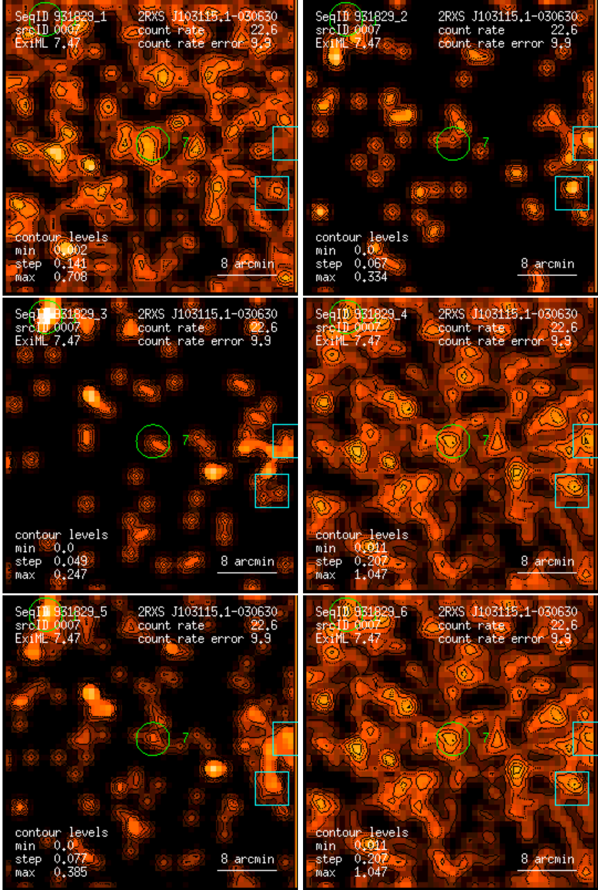
Figure 7: RASS 931829: detection 0007: band rate images, Gaussian filter: (1) PSPC channels 11 – 41, (2) 52 – 90, (3) 91 – 201, (4) 11 – 235, (5) 52 – 201, (6) 11 – 201. Broad band rates in counts/ks. Band rate contour levels in counts/ks/arcmin 2 .
