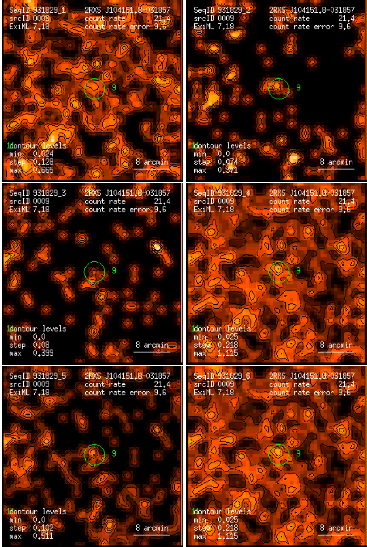
Figure 9: RASS 931829: detection 0009: band rate images, Gaussian filter: (1) PSPC channels 11 – 41, (2) 52 – 90, (3) 91 – 201, (4) 11 – 235, (5) 52 – 201, (6) 11 – 201. Broad band rates in counts/ks. Band rate contour levels in counts/ks/arcmin 2 .
