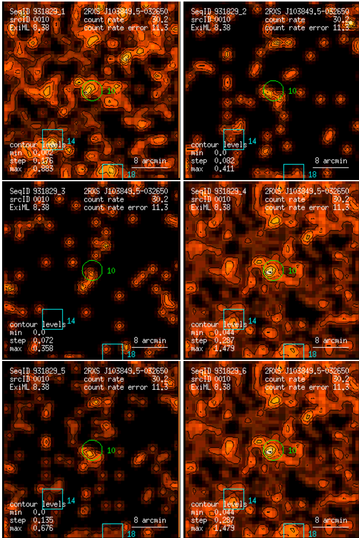
Figure 10: RASS 931829: detection 0010: band rate images, Gaussian filter: (1) PSPC channels 11 – 41, (2) 52 – 90, (3) 91 – 201, (4) 11 – 235, (5) 52 – 201, (6) 11 – 201. Broad band rates in counts/ks. Band rate contour levels in counts/ks/arcmin 2 .
