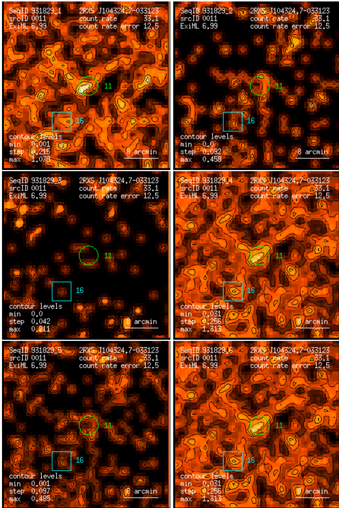
Figure 11: RASS 931829: detection 0011: band rate images, Gaussian filter: (1) PSPC channels 11 – 41, (2) 52 – 90, (3) 91 – 201, (4) 11 – 235, (5) 52 – 201, (6) 11 – 201. Broad band rates in counts/ks. Band rate contour levels in counts/ks/arcmin 2 .
